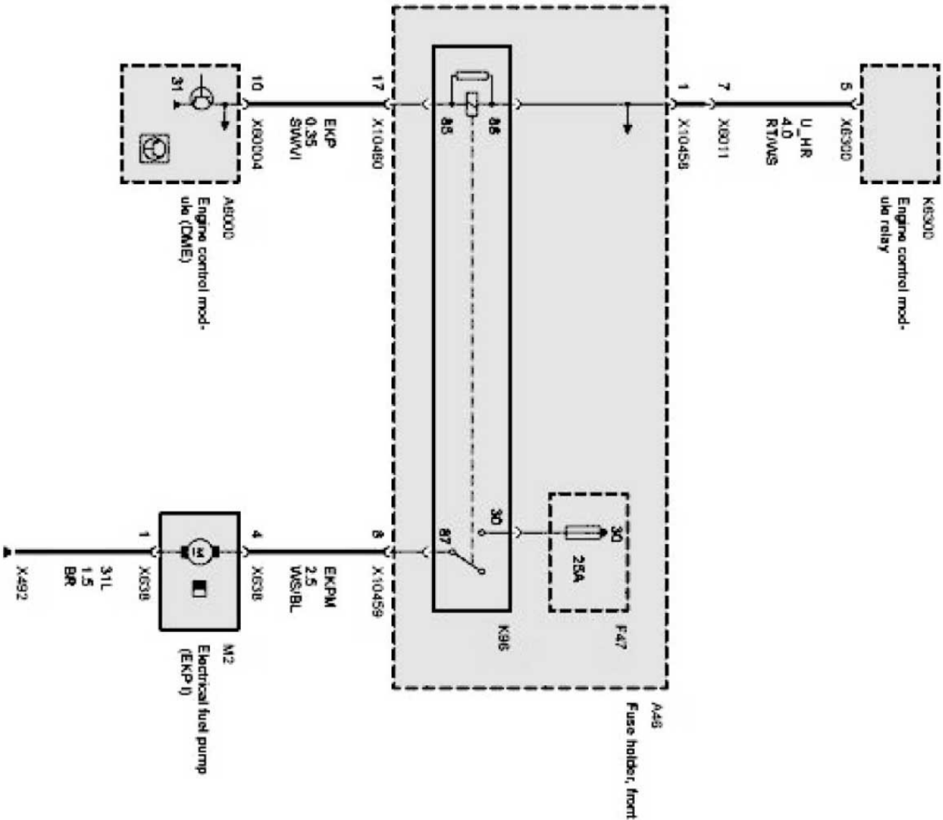
E53 Fuel pump Part 1 Of 1
