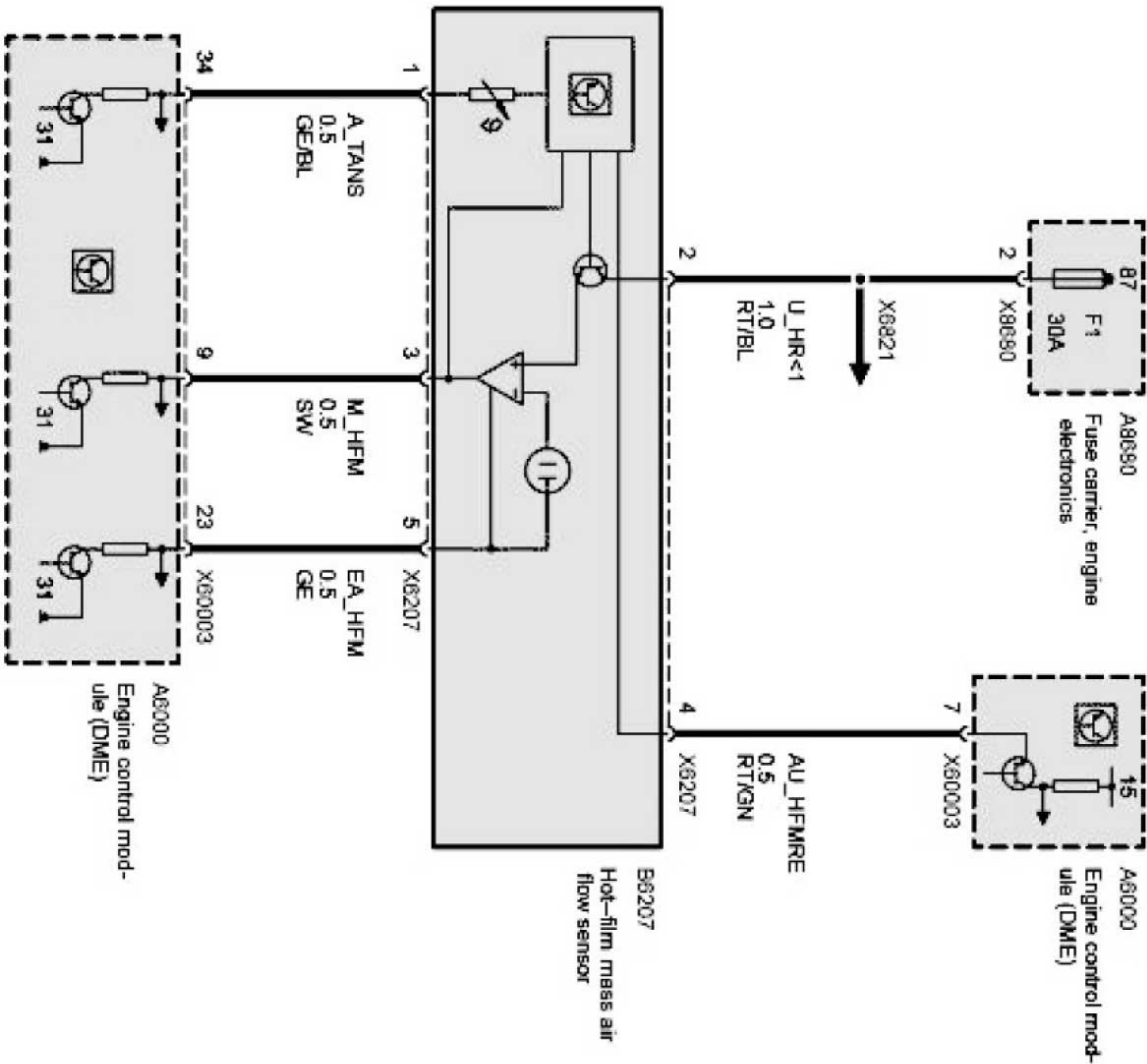
E53 Hot-film mass air flow sensor Part 1 Of 1
