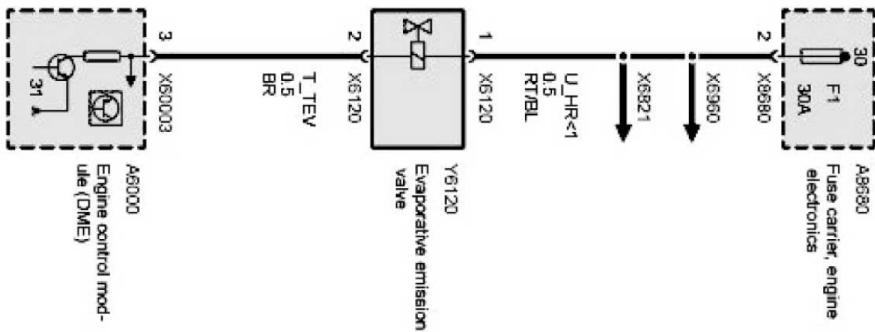
E53 Tank ventilation valve Part 1 Of 1
