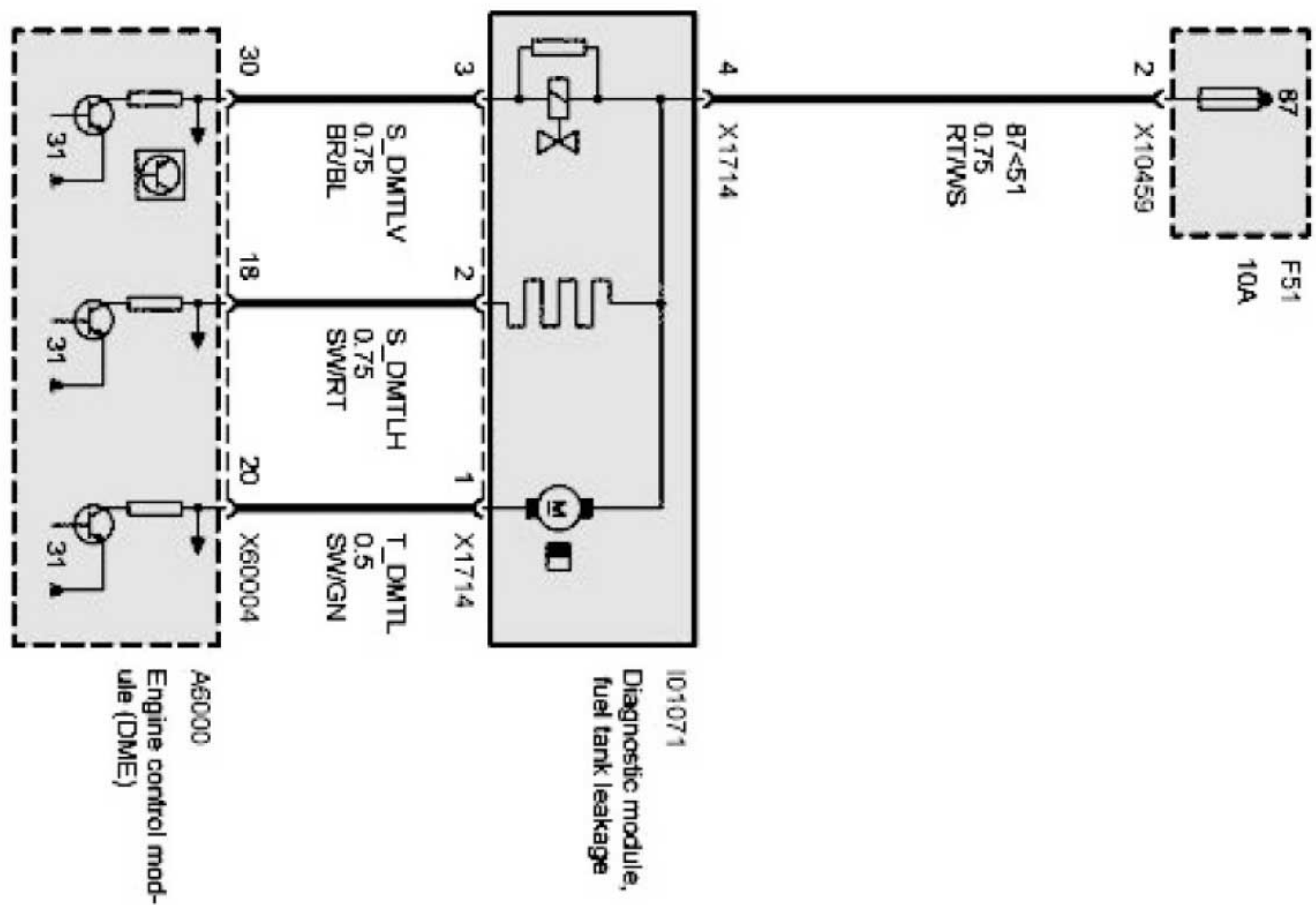
E53 Diagnosis module, tank leakage Part 1 Of 1
