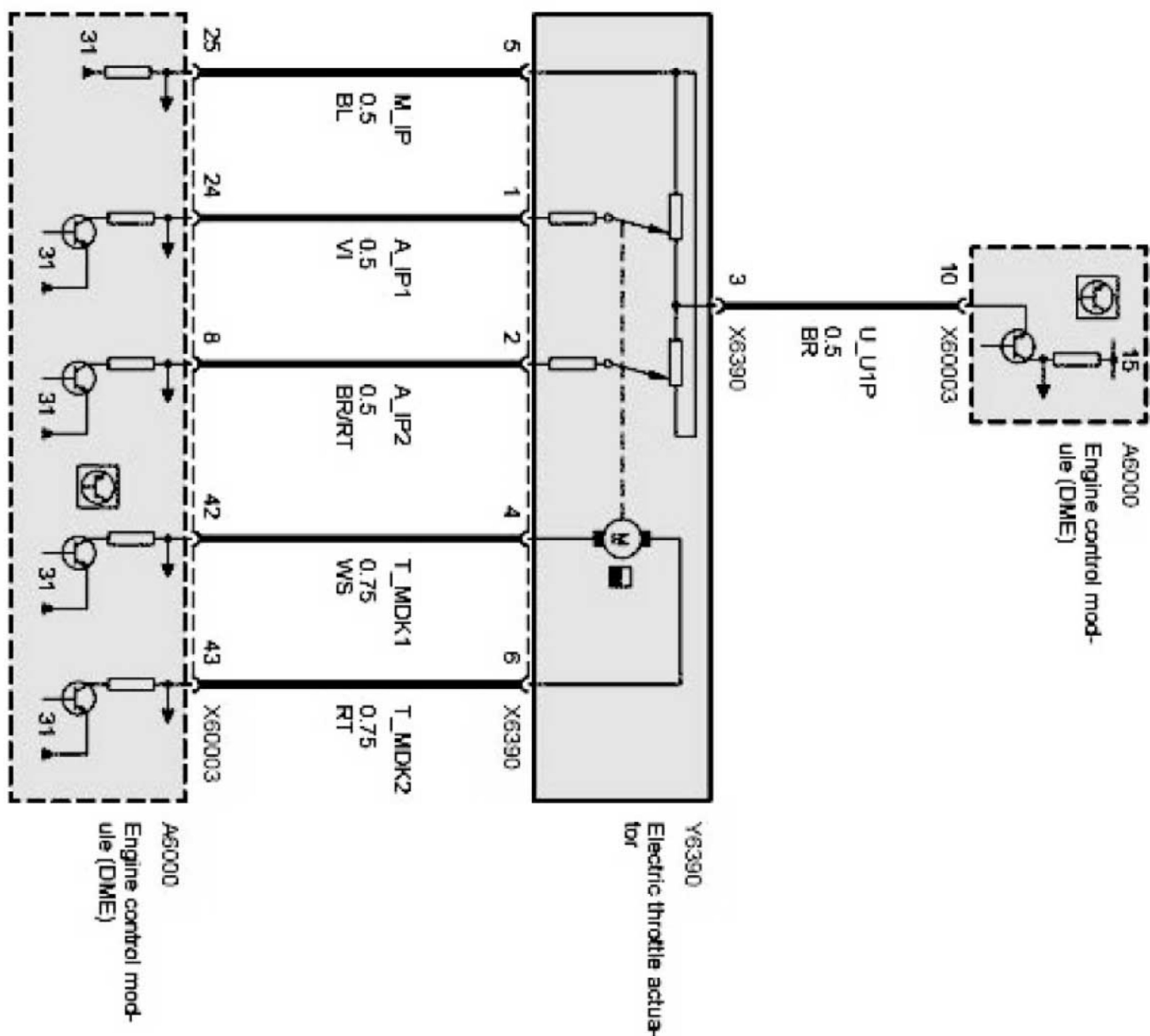
E53 Electric throttle actuator Part 1 Of 1
