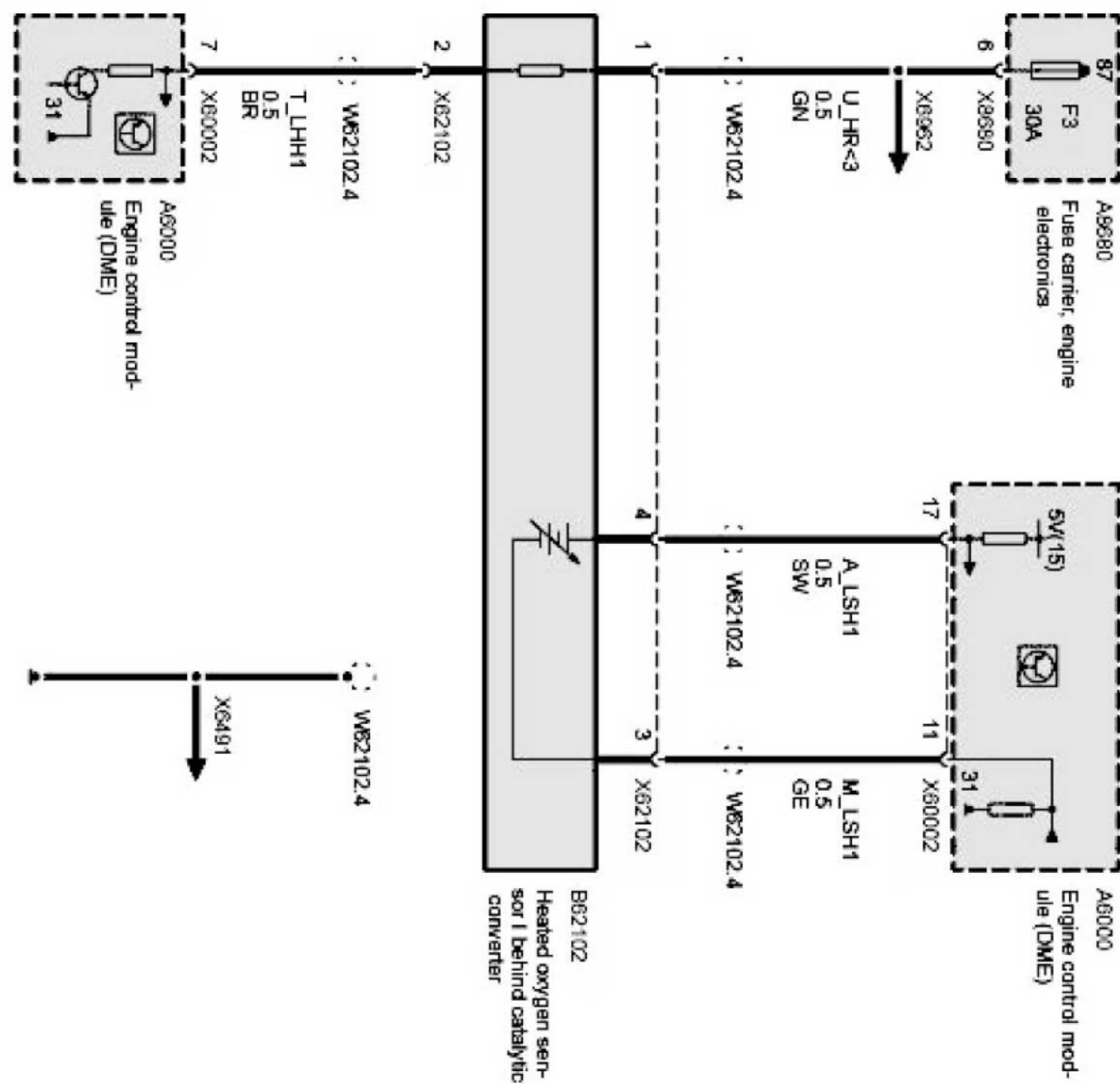
E53 Oxygen sensor I behind catalytic converter Part 1 Of 1
