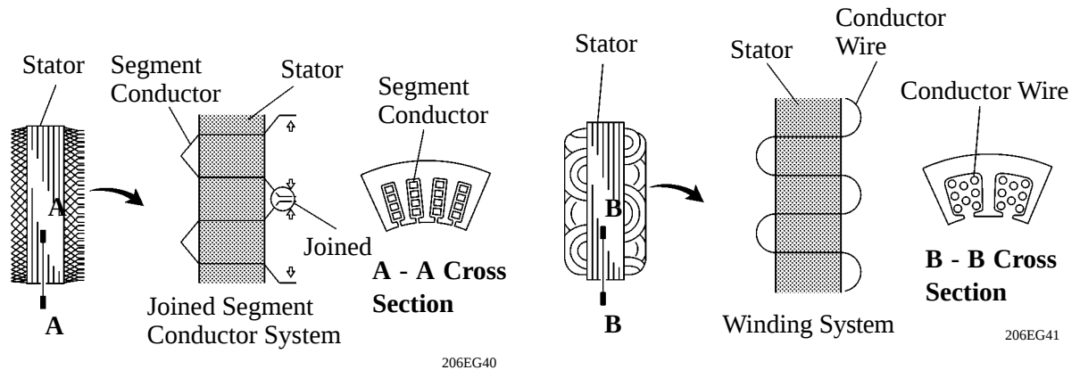
Conventional Type Generator
