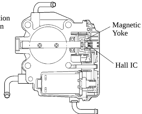
Cross Section
