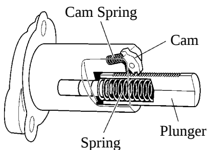
Chain Tensioner
