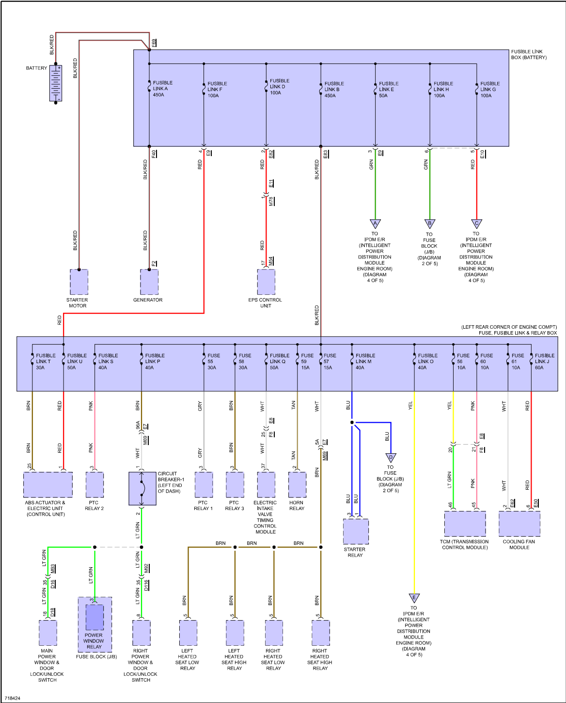
Fig 1: Power Distribution Circuit (1 of 5)
