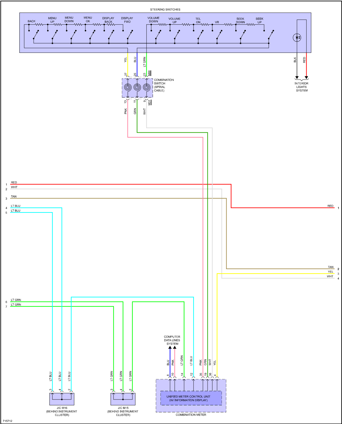
Fig 7: Navigation Circuit, W/O Bose (2 of 3)
