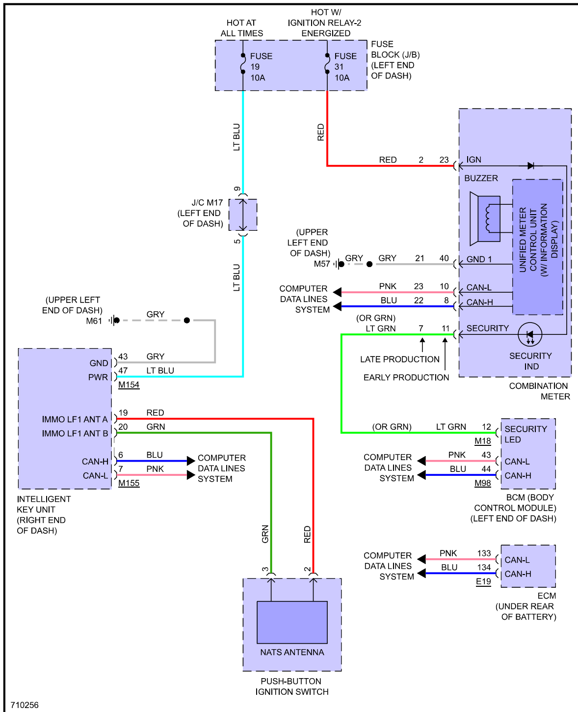
Fig 5: Immobilizer Circuit
