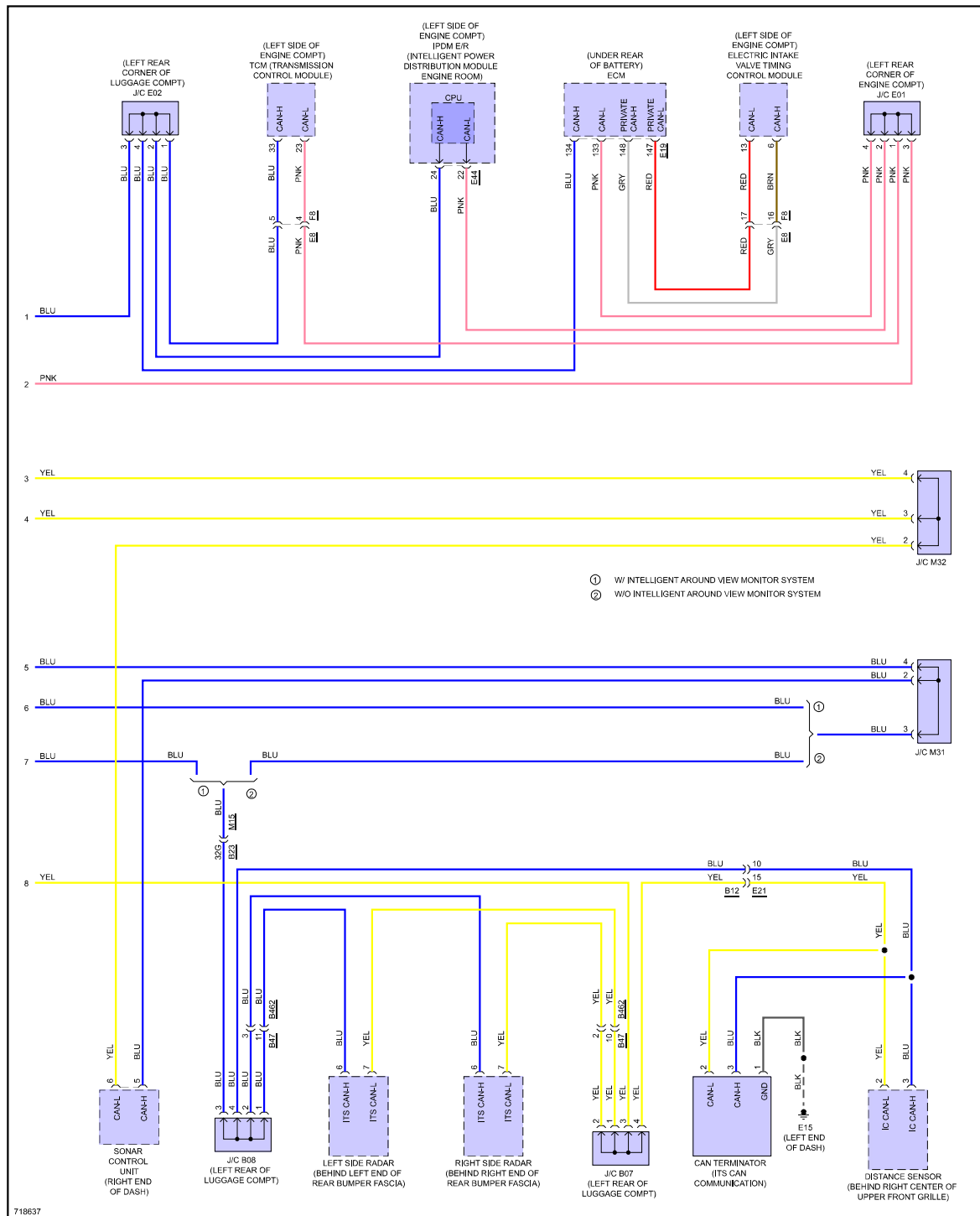
Fig 4: Computer Data Lines Circuit (4 of 4)
