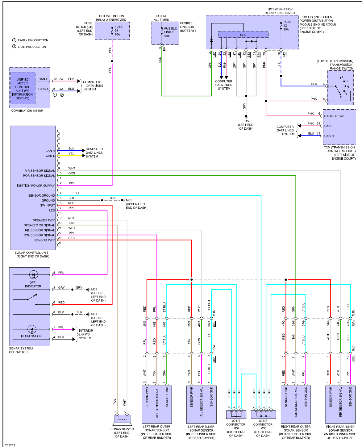
Fig 10: Sonar Circuit
