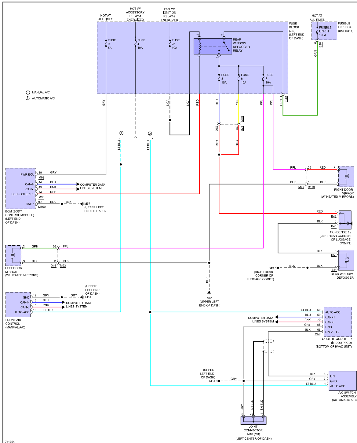
Fig 1: Defoggers Circuit
