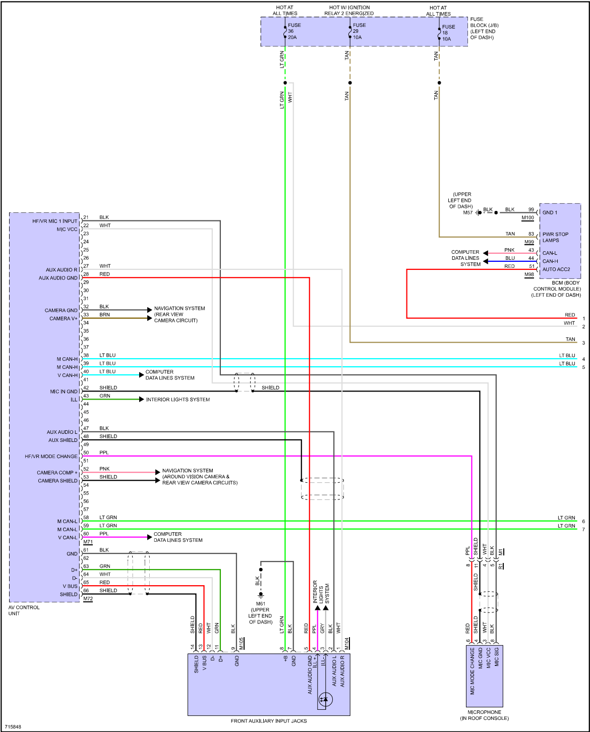
Fig 6: Premium Radio Circuit, W/O Bose (1 of 3)
