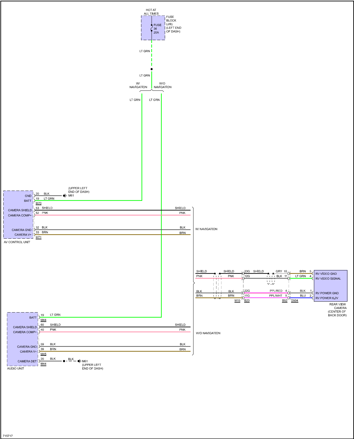
Fig 9: Rear View Camera Circuit
