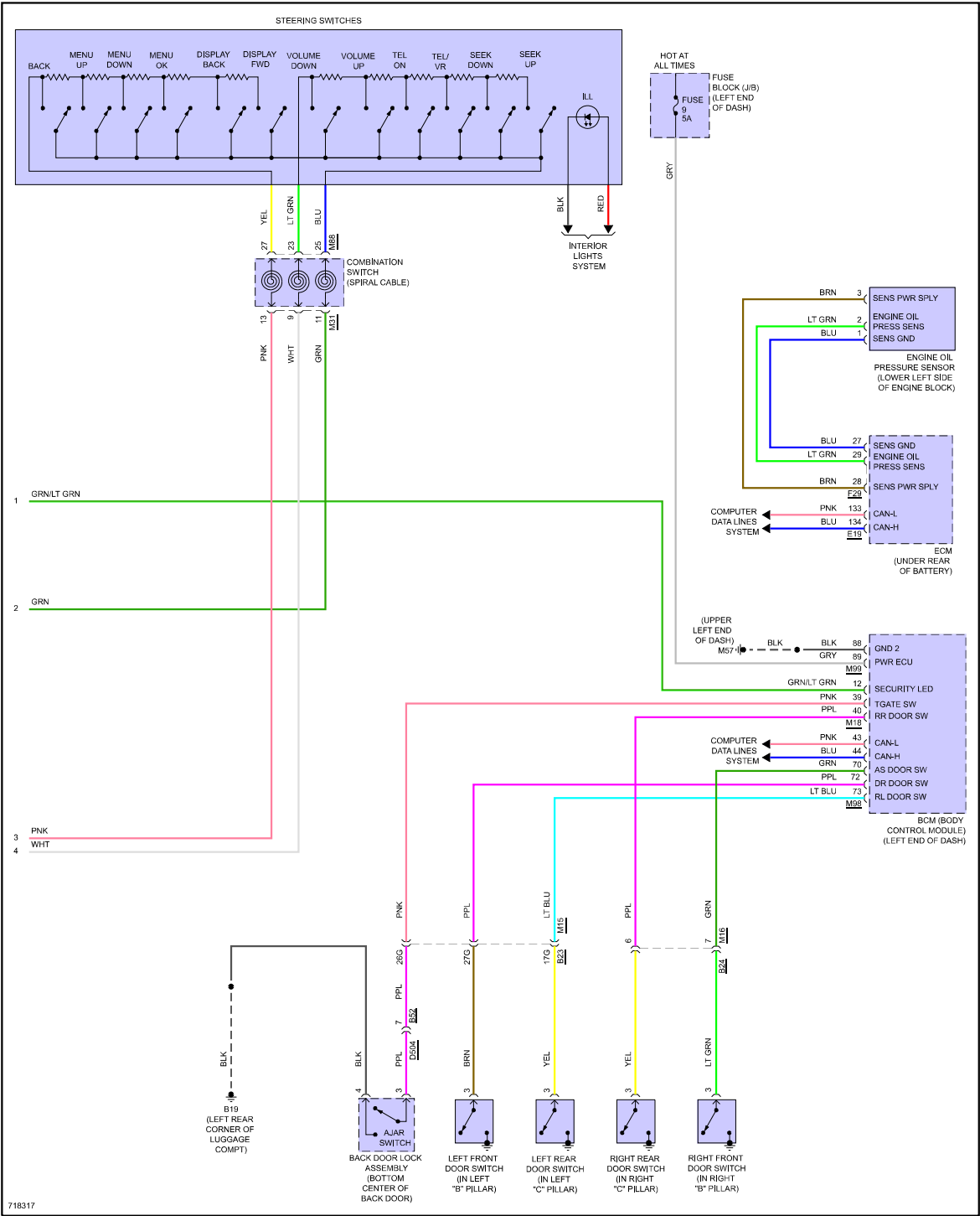
Fig 2: Instrument Cluster Circuit, Early Production (2 of 2)
