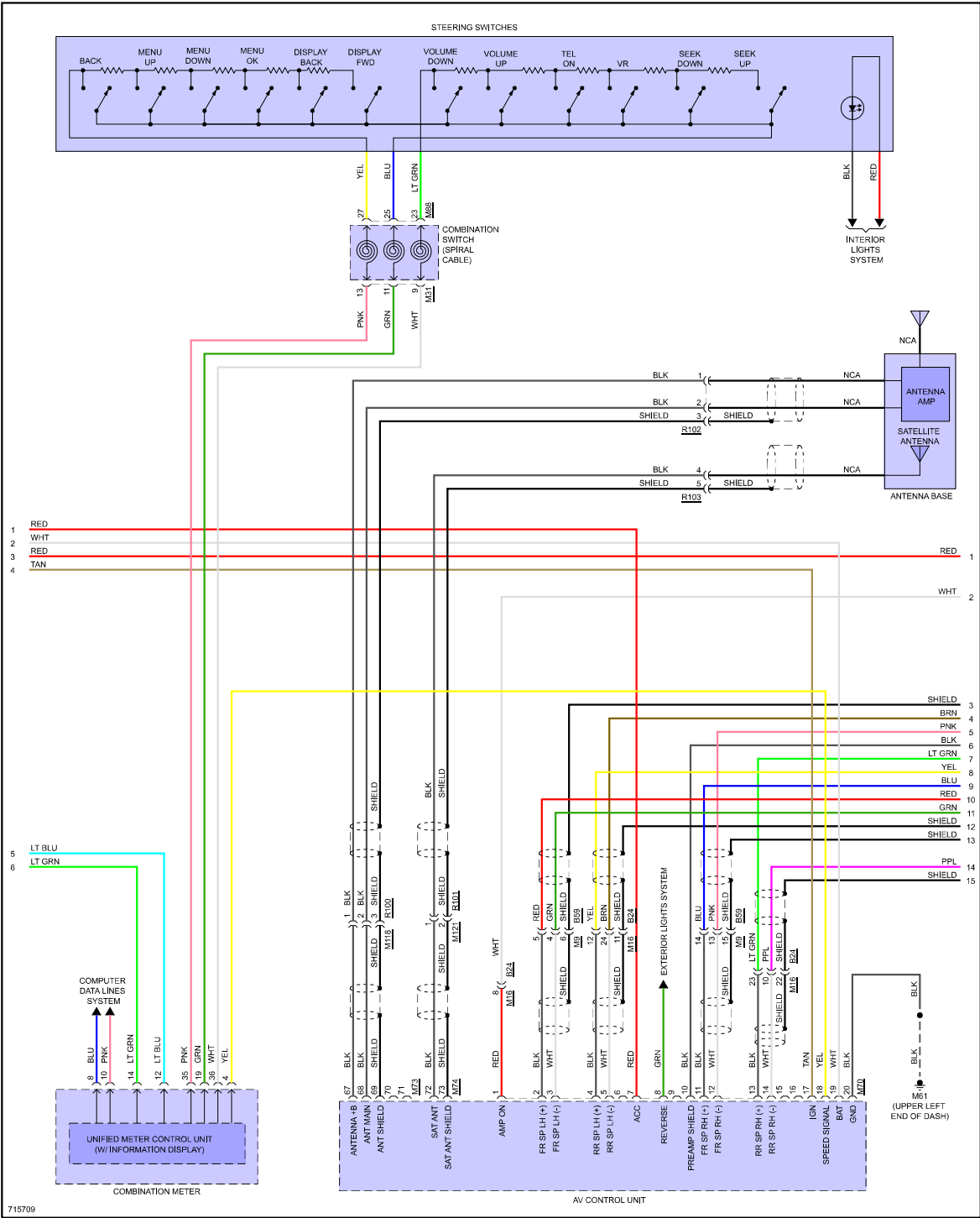
Fig 4: Navigation Circuit, W/ Bose (2 of 3)
