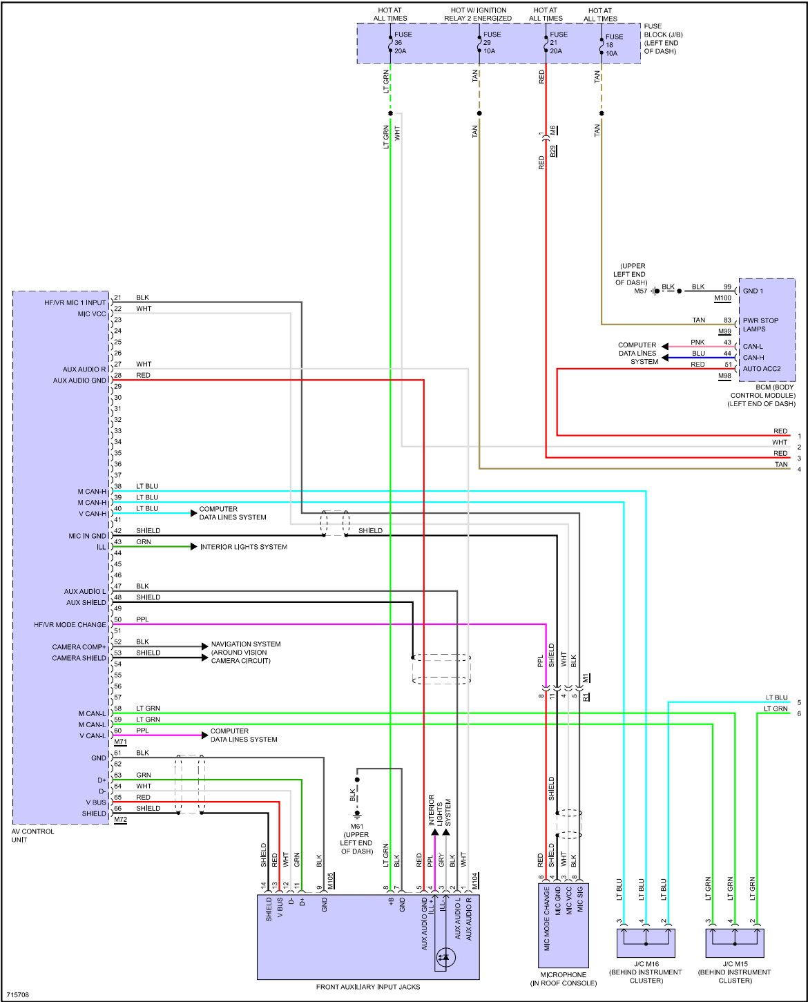
Fig 3: Navigation Circuit, W/ Bose (1 of 3)
