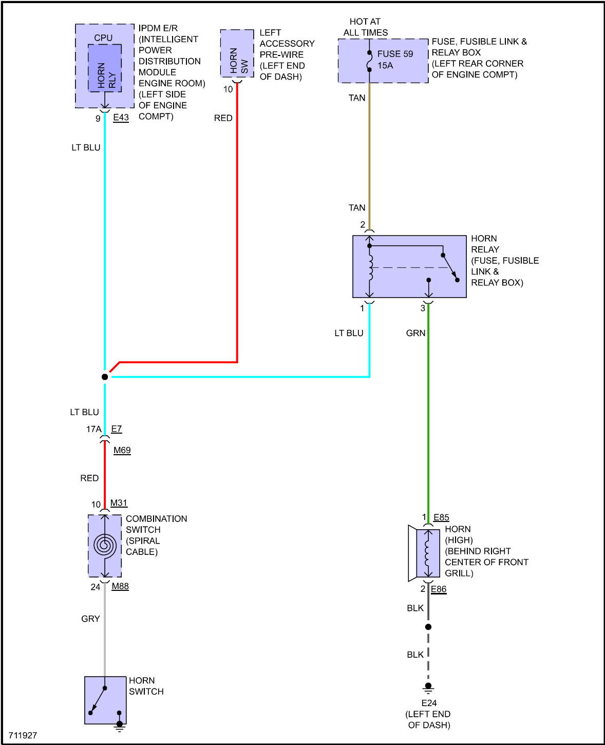
Fig 1: Horn Circuit
