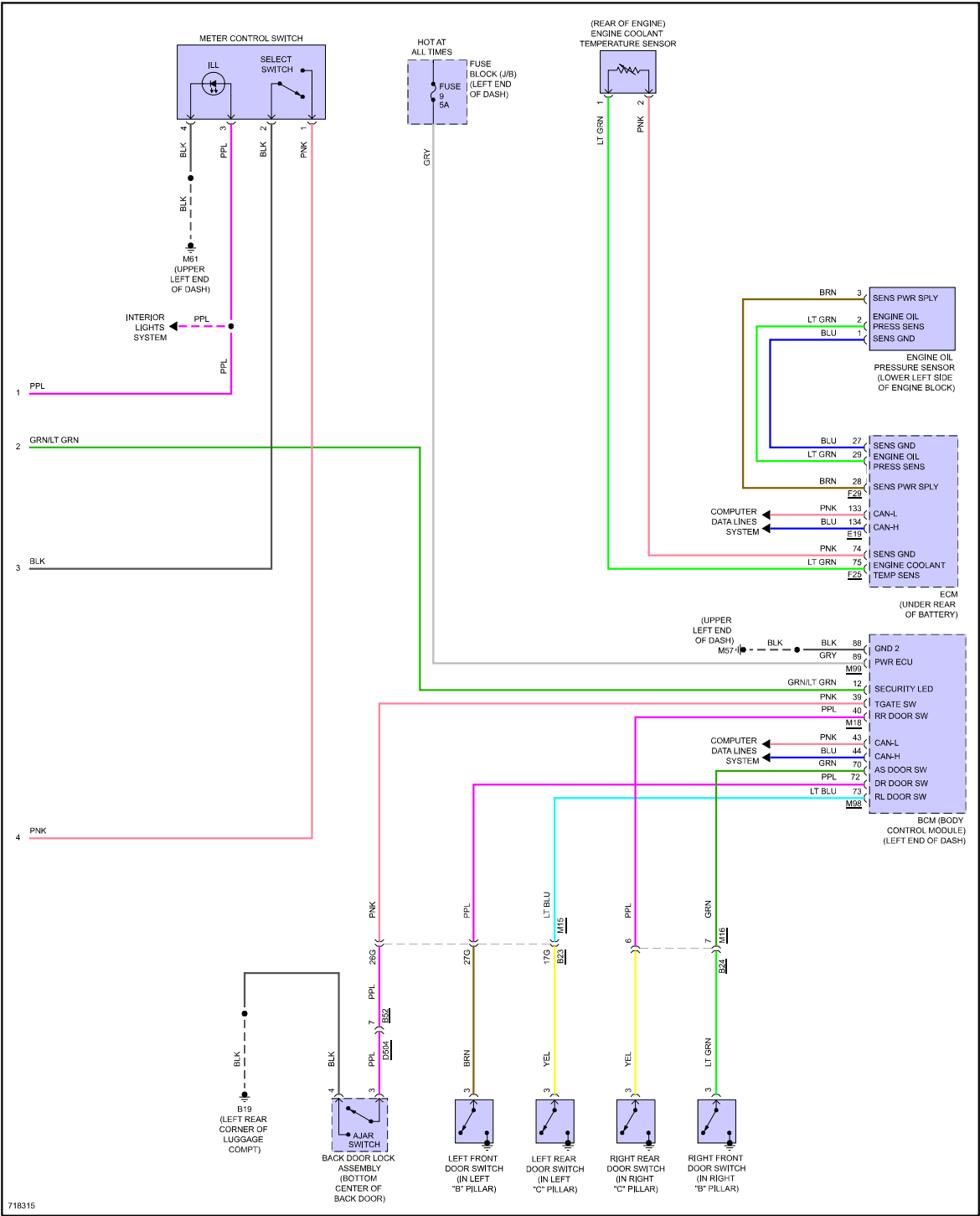
Fig 4: Instrument Cluster Circuit, Late Production (2 of 2)
