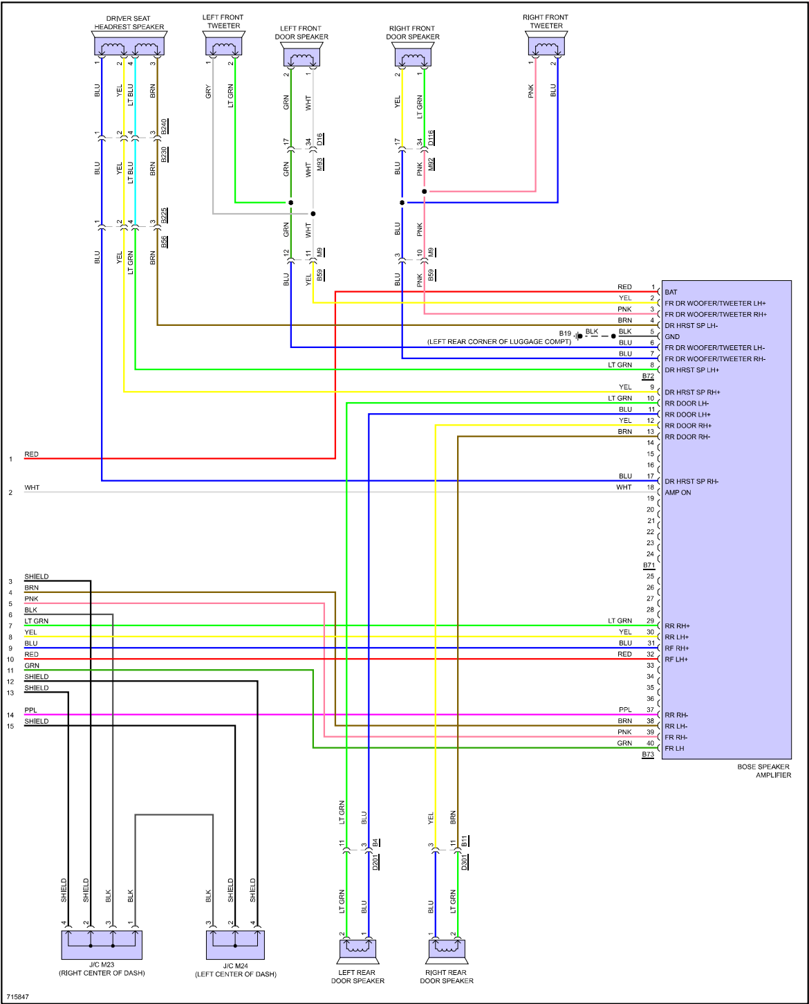
Fig 5: Premium Radio Circuit, W/ Bose (3 of 3)
