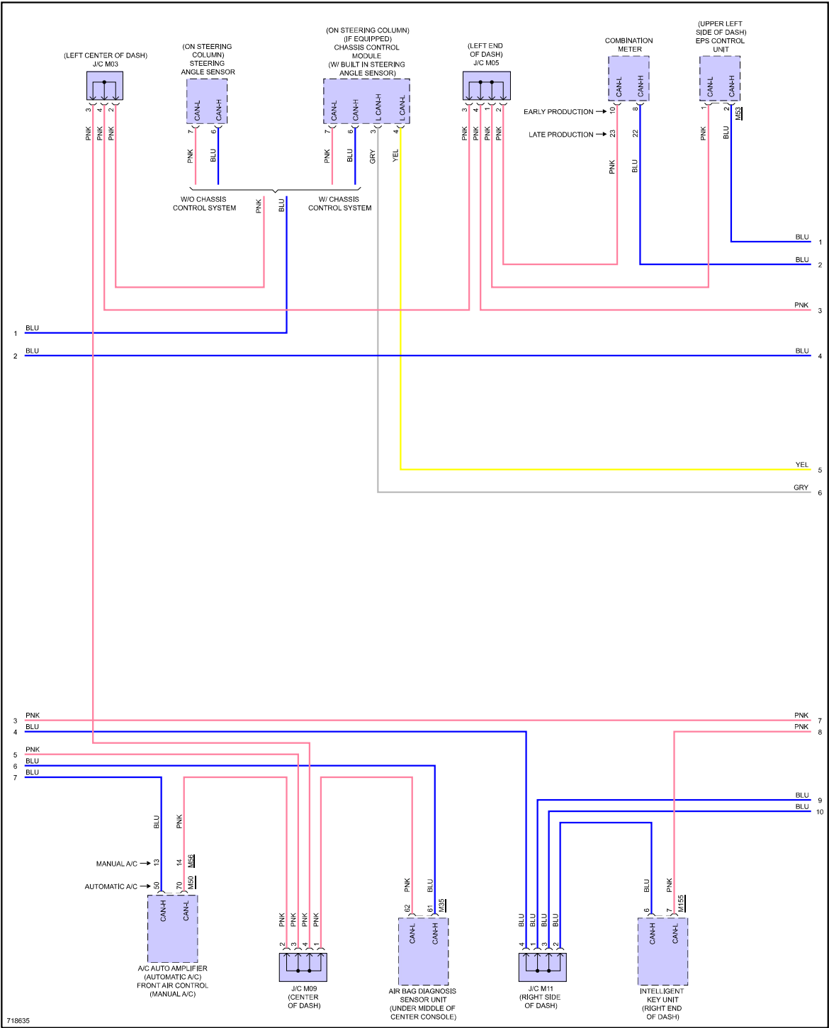
Fig 2: Computer Data Lines Circuit (2 of 4)
