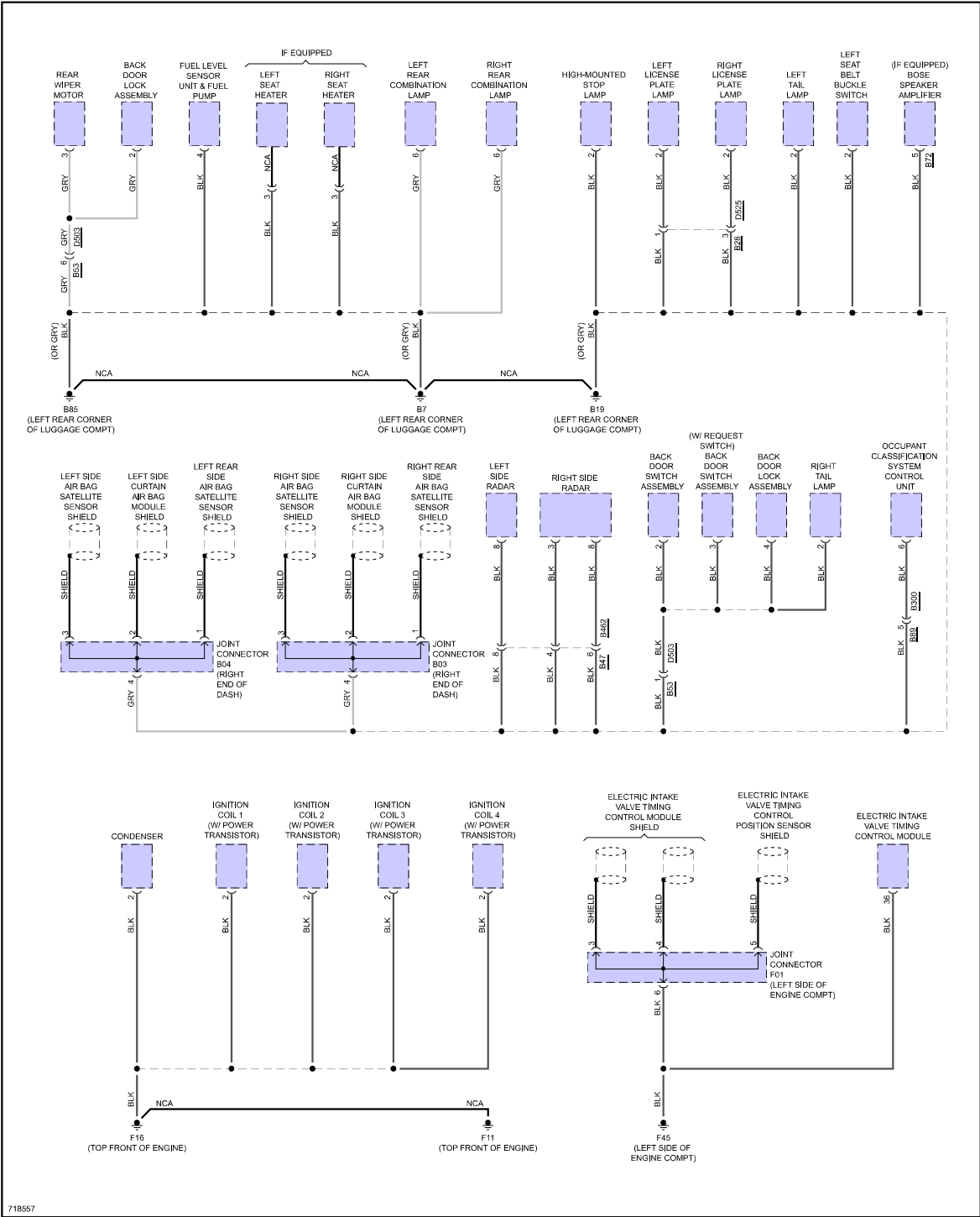
Fig 1: Ground Distribution Circuit (1 of 4)
