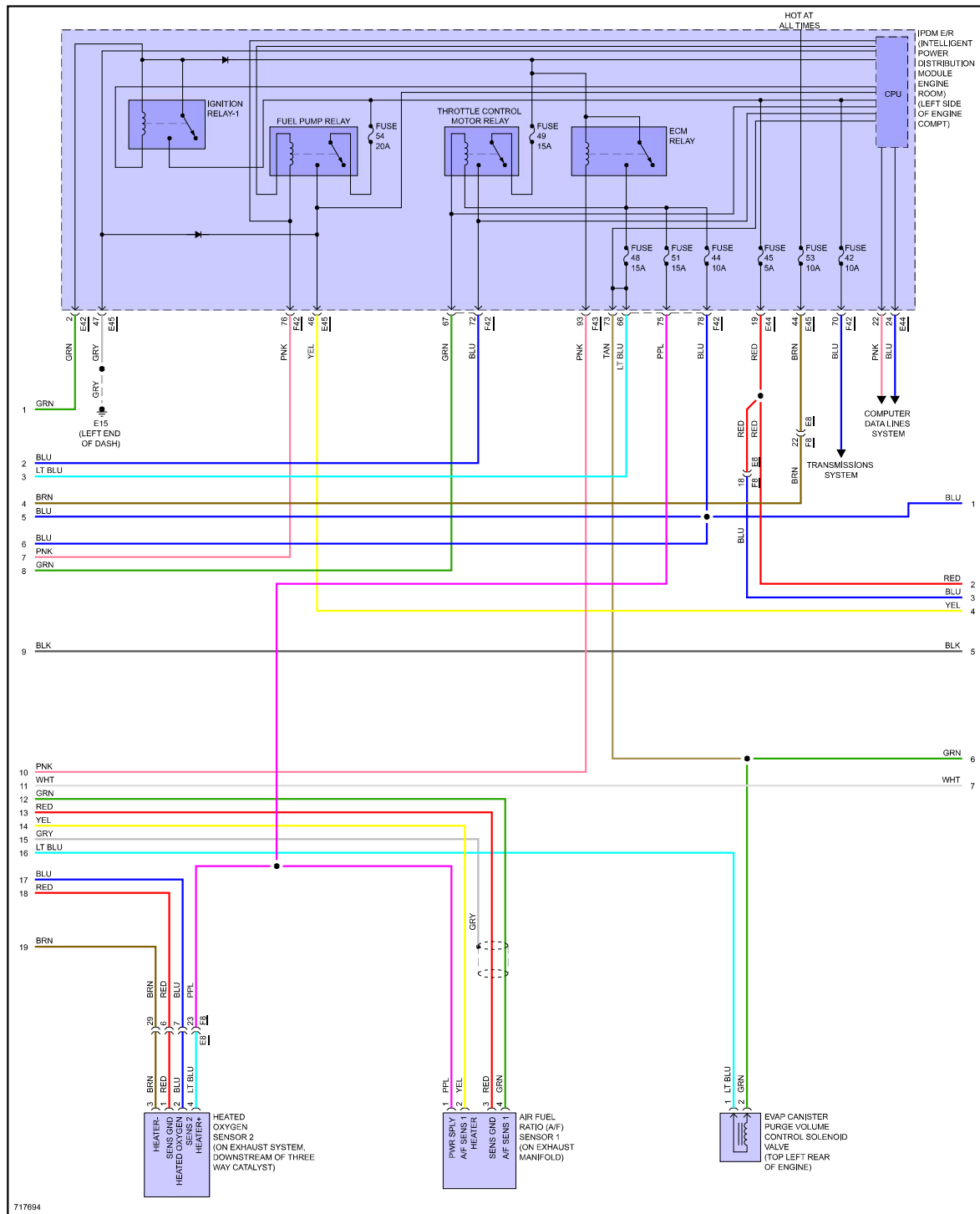
Fig 4: 1.6L, Engine Performance Circuit (4 of 6)
