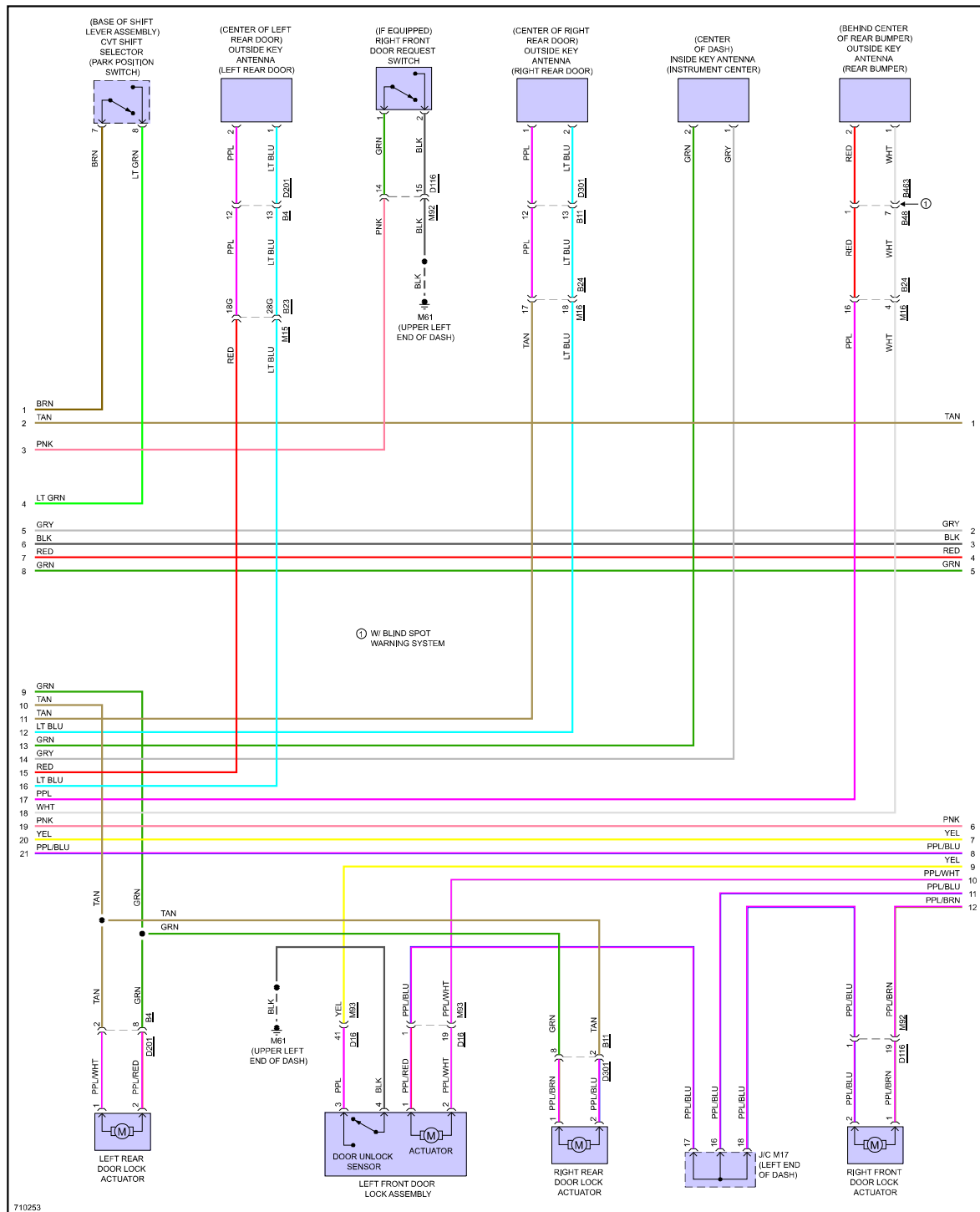
Fig 2: Forced Entry Circuit (2 of 4)
