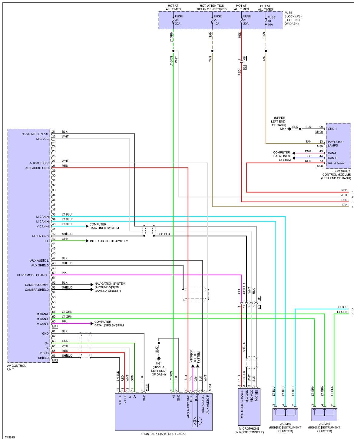
Fig 3: Premium Radio Circuit, W/ Bose (1 of 3)
