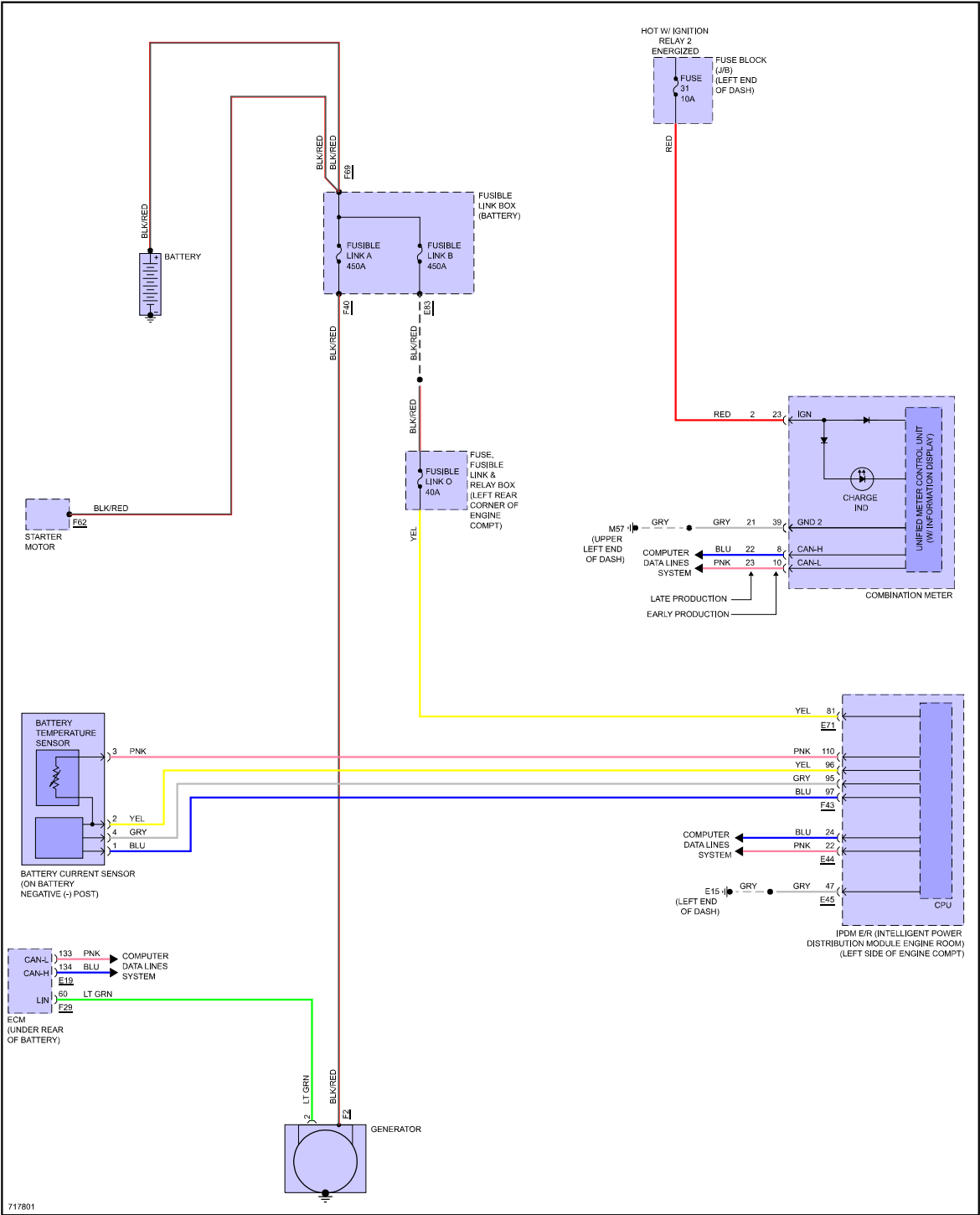
Fig 1: Charging Circuit
