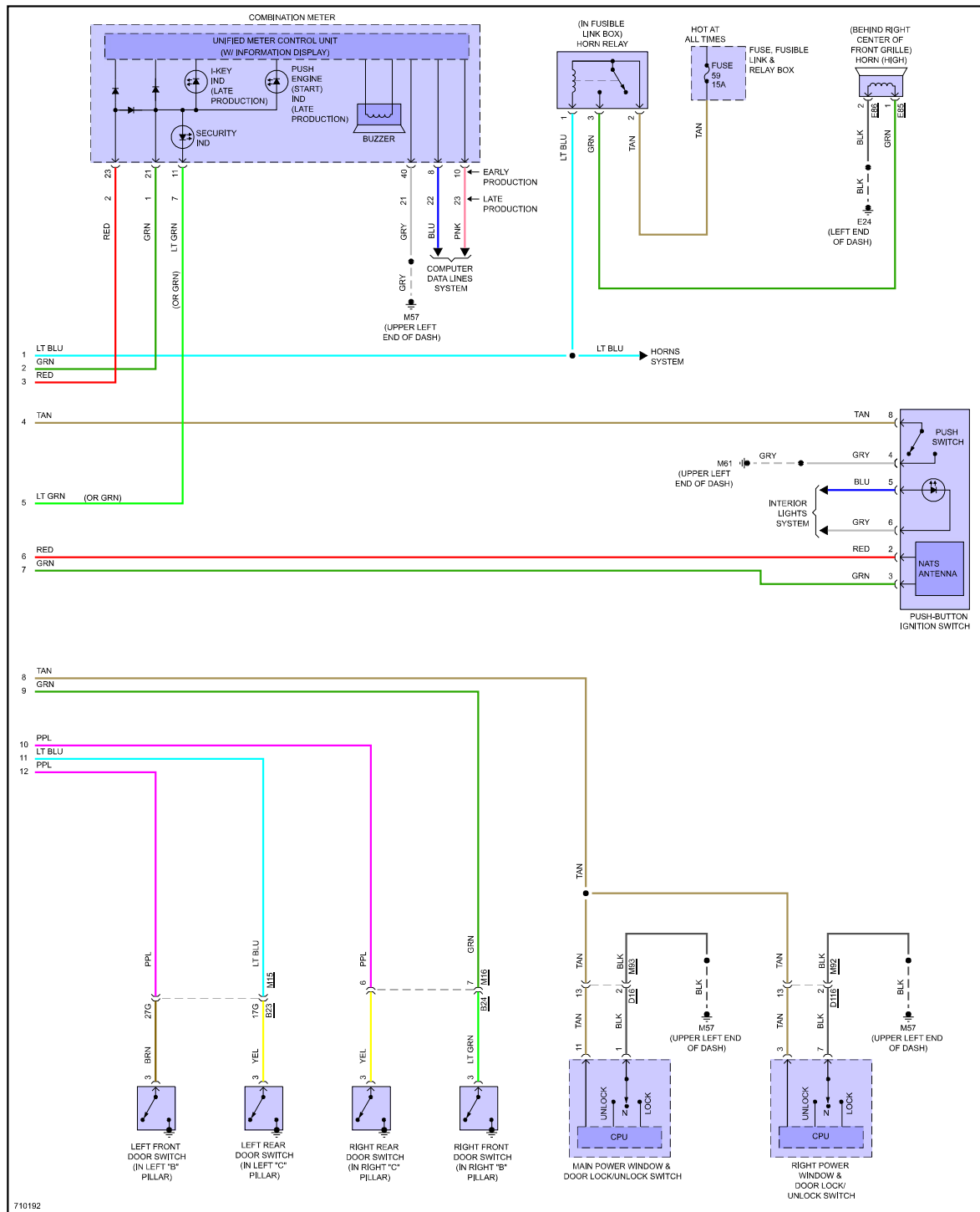
Fig 4: Power Door Locks Circuit (4 of 4)
