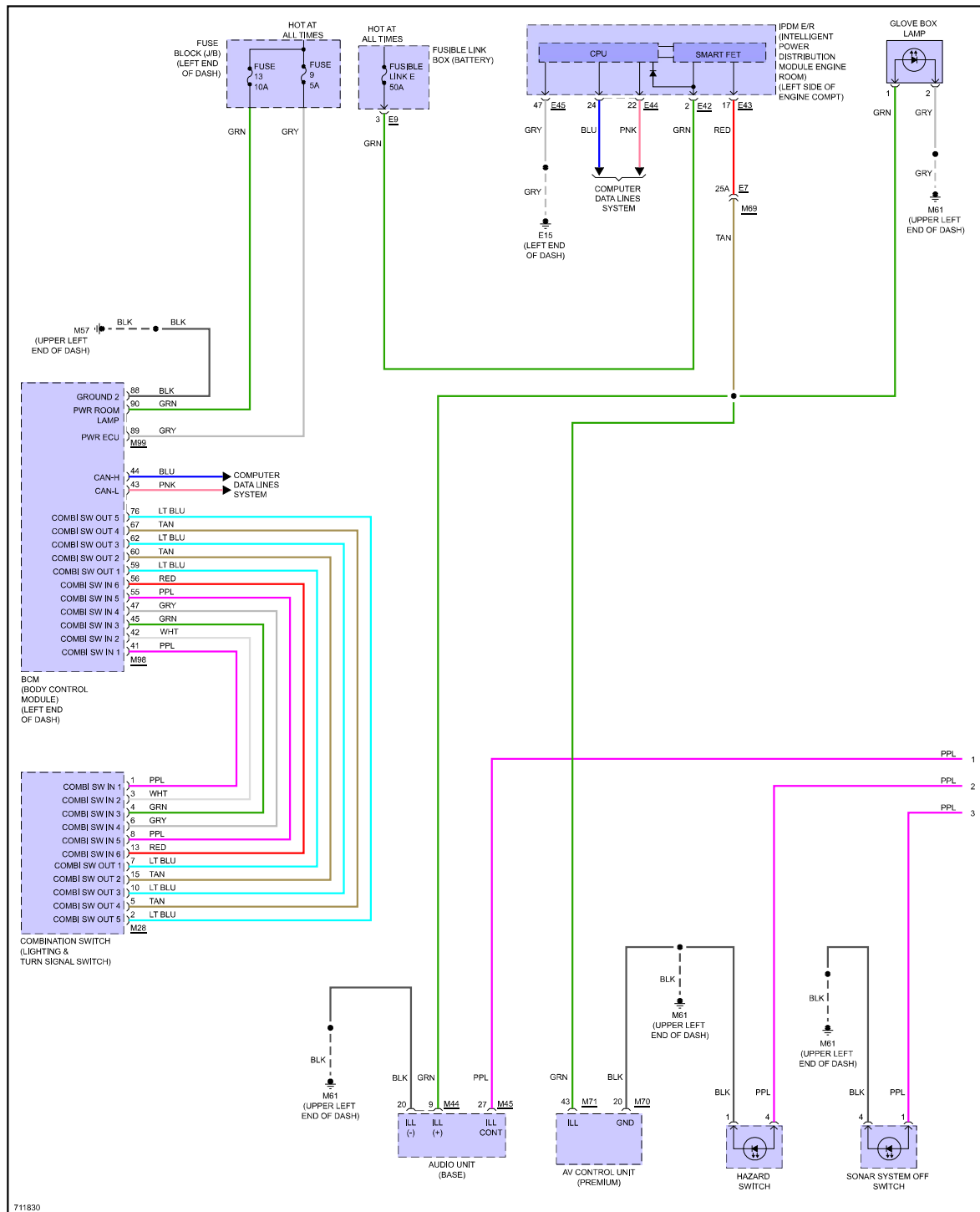
Fig 2: Instrument Illumination Circuit (1 of 2)
