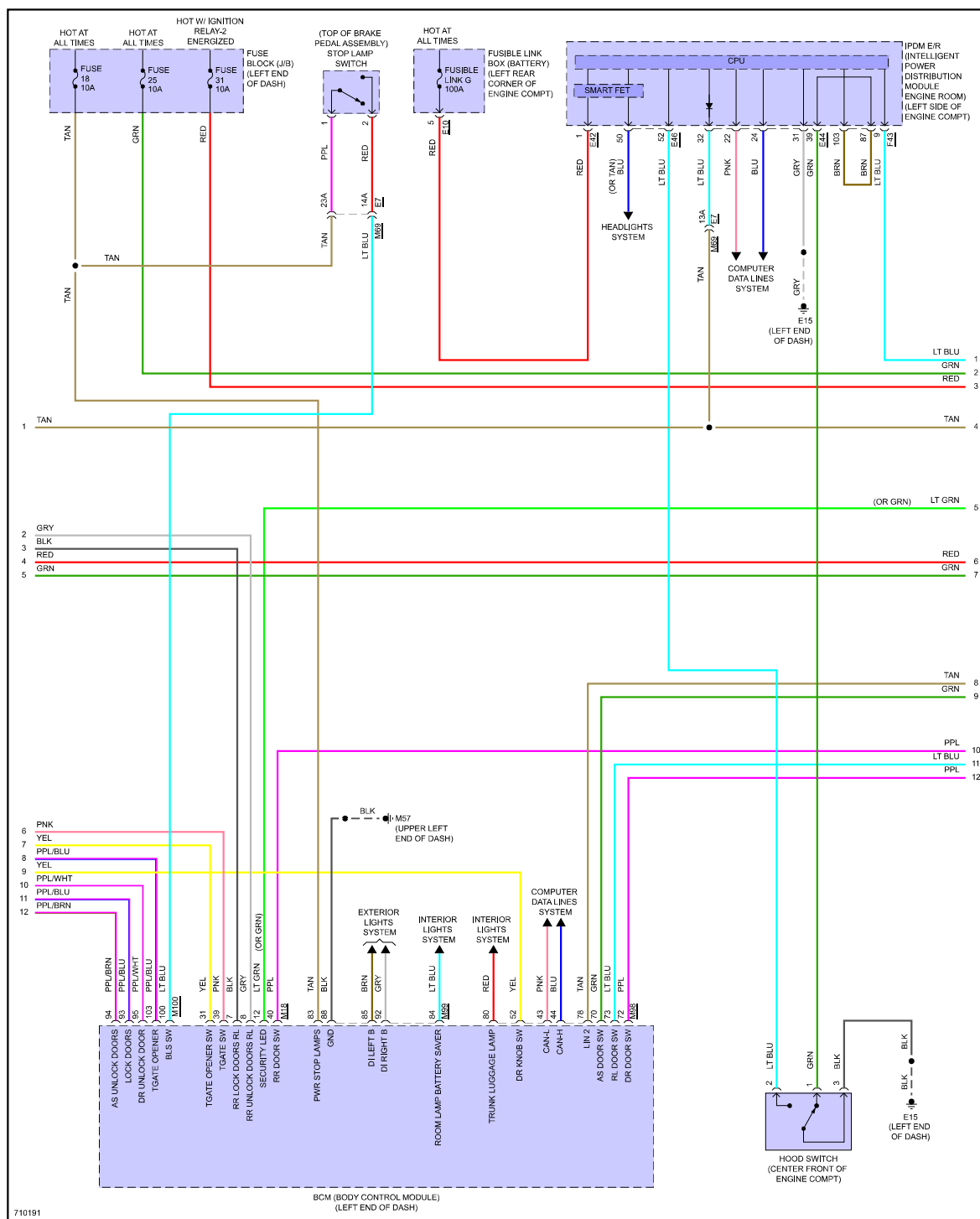
Fig 3: Power Door Locks Circuit (3 of 4)
