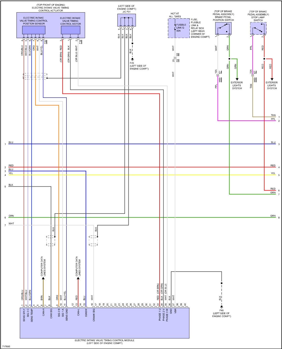
Fig 5: 1.6L, Engine Performance Circuit (5 of 6)
