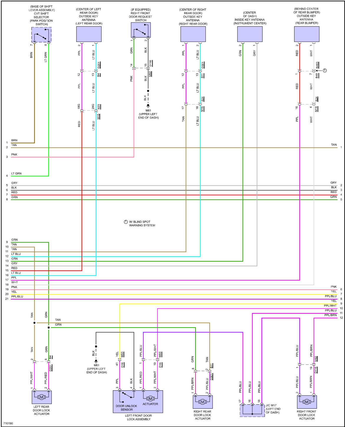
Fig 2: Power Door Locks Circuit (2 of 4)
