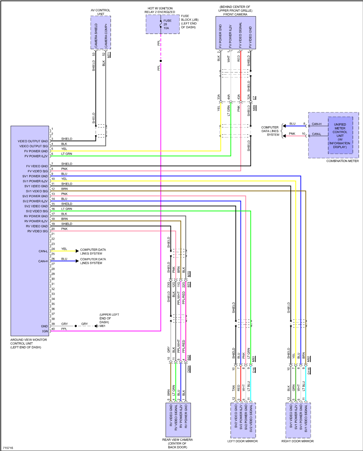
Fig 1: Around Vision Camera Circuit
