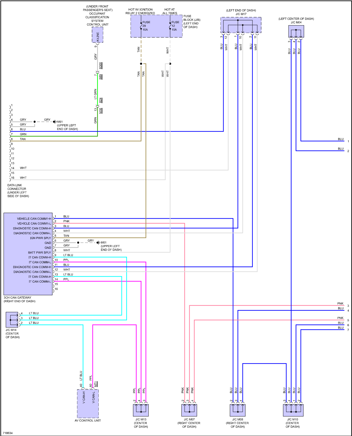
Fig 1: Computer Data Lines Circuit (1 of 4)
