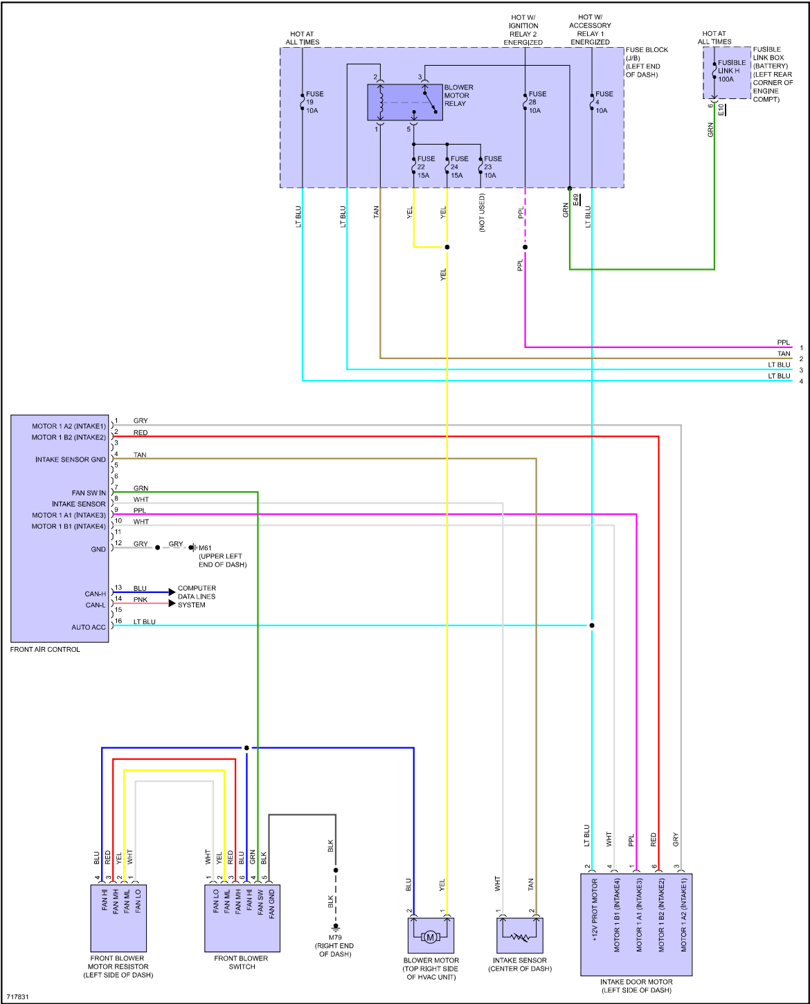
Fig 5: Manual A/C Circuit (1 of 3)
