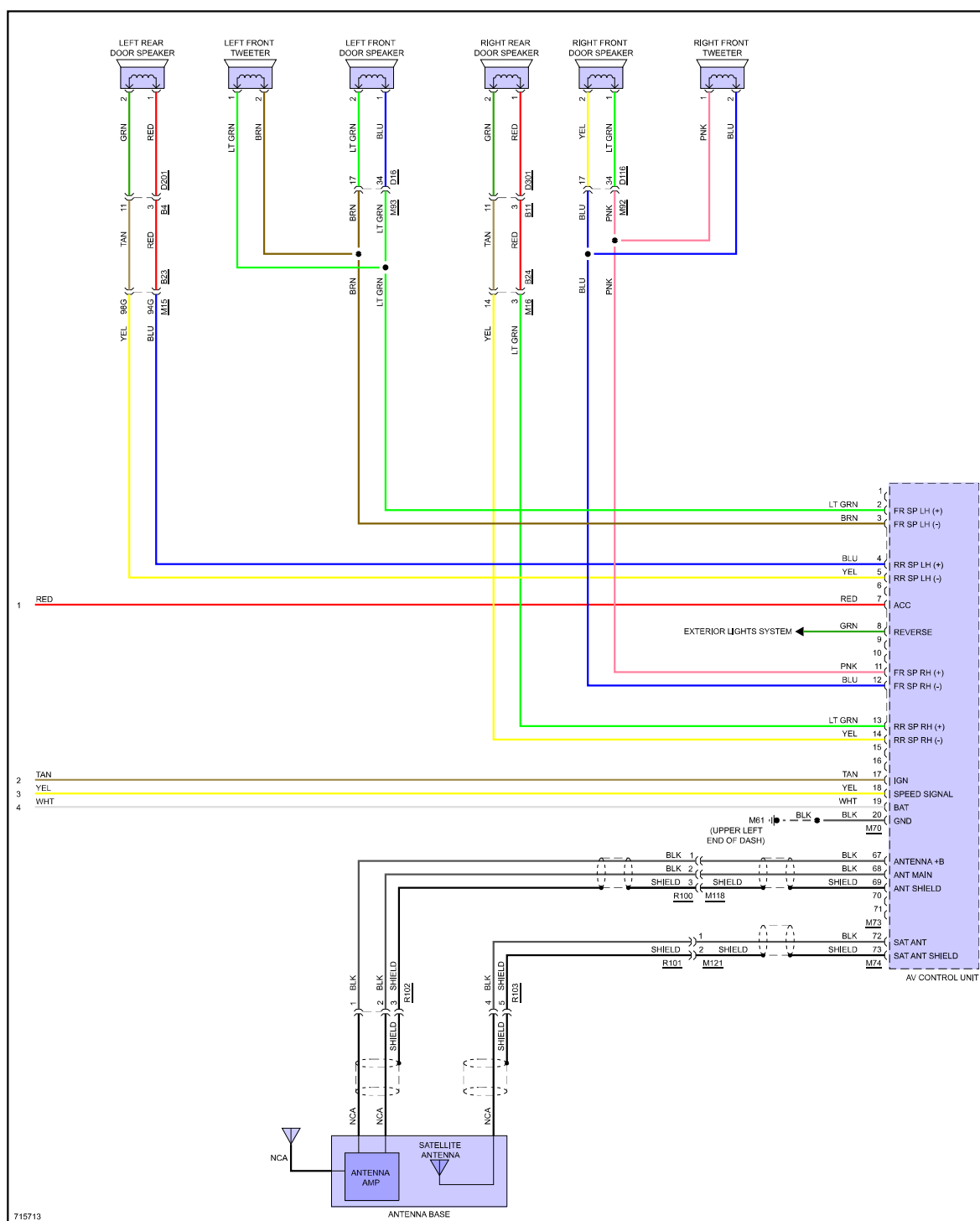
Fig 8: Navigation Circuit, W/O Bose (3 of 3)
