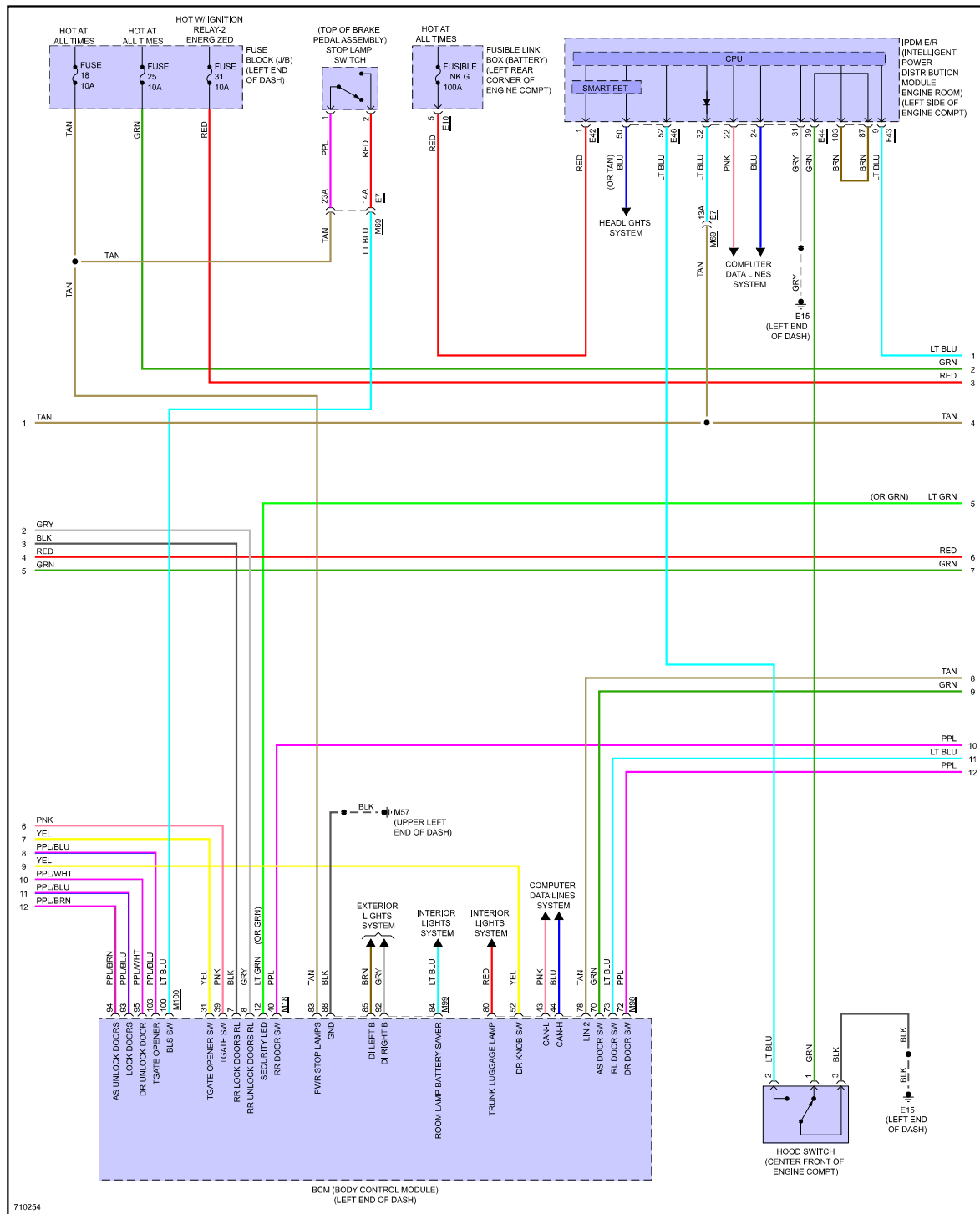
Fig 3: Forced Entry Circuit (3 of 4)
