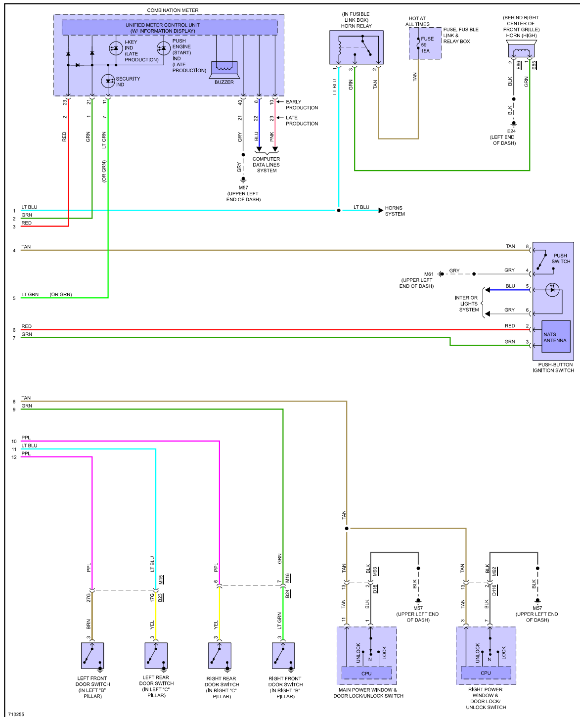
Fig 4: Forced Entry Circuit (4 of 4)
