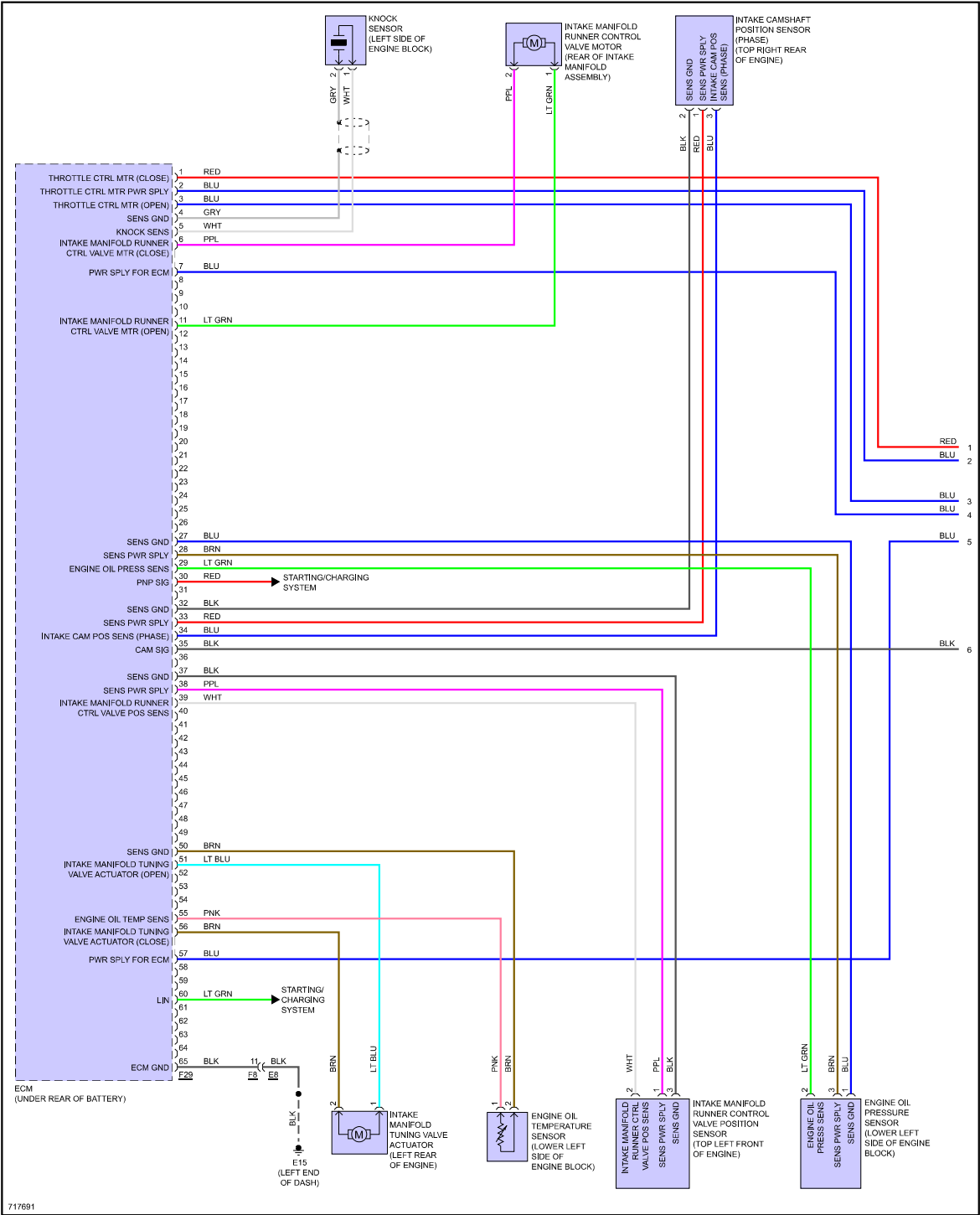
Fig 1: 1.6L, Engine Performance Circuit (1 of 6)
