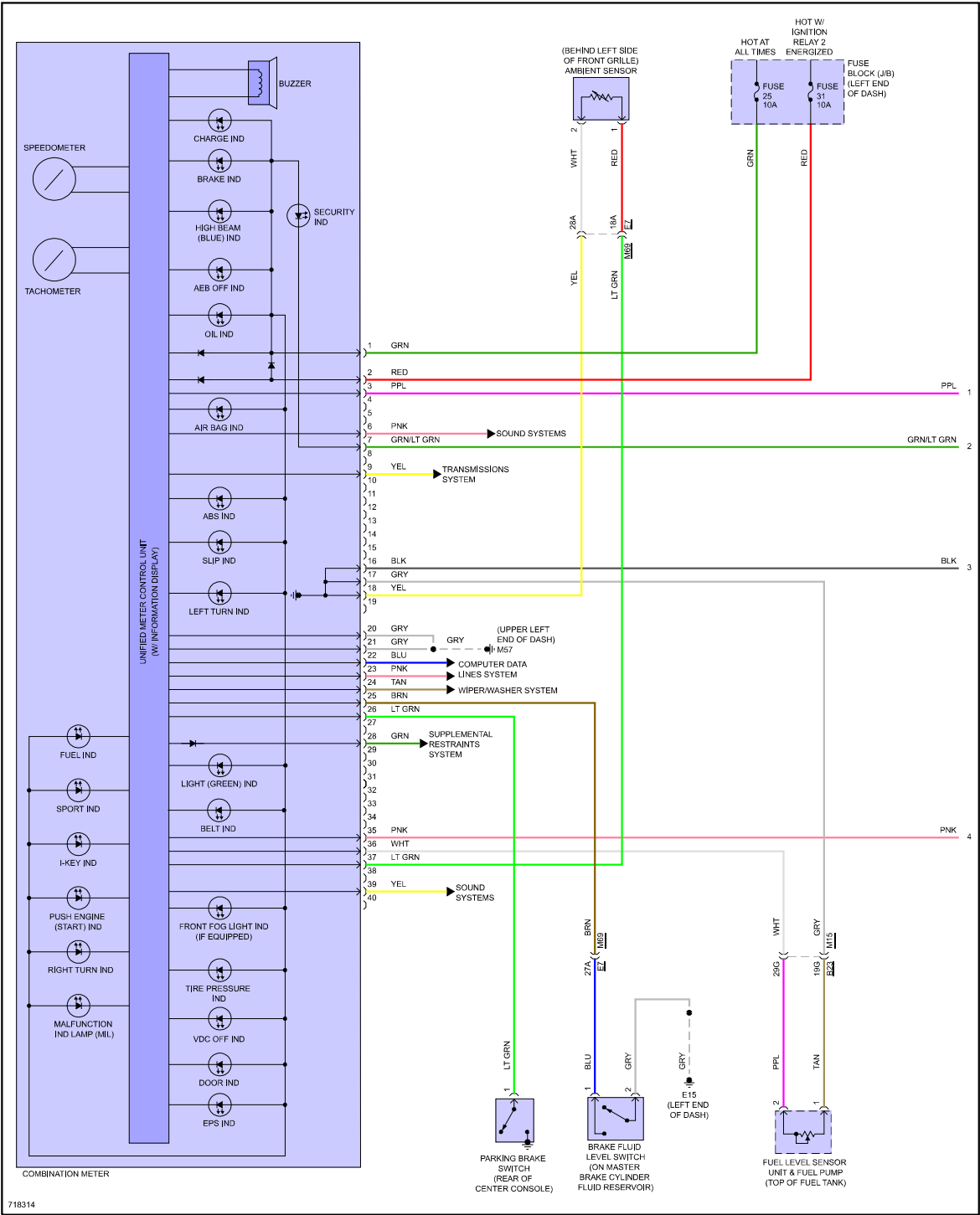
Fig 3: Instrument Cluster Circuit, Late Production (1 of 2)
