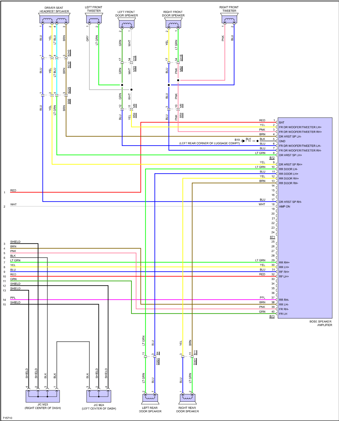
Fig 5: Navigation Circuit, W/ Bose (3 of 3)
