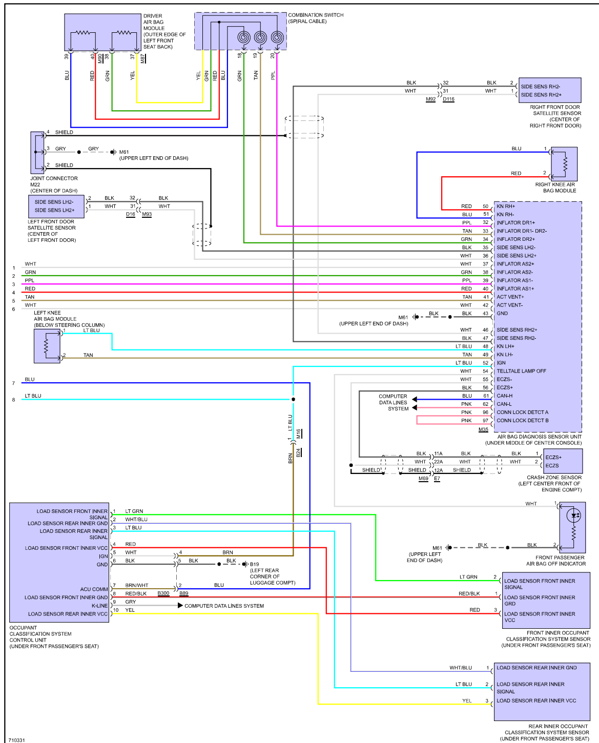
Fig 3: Supplemental Restraints Circuit (3 of 3)
