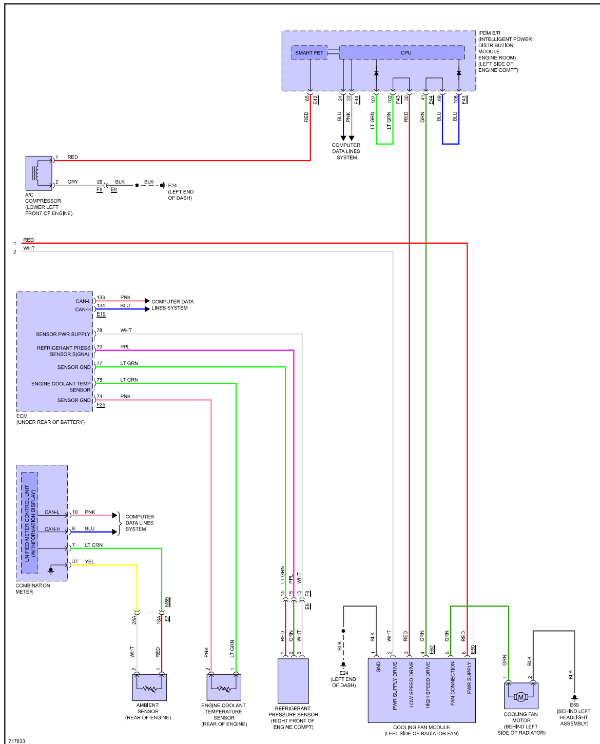
Fig 7: Manual A/C Circuit (3 of 3)
