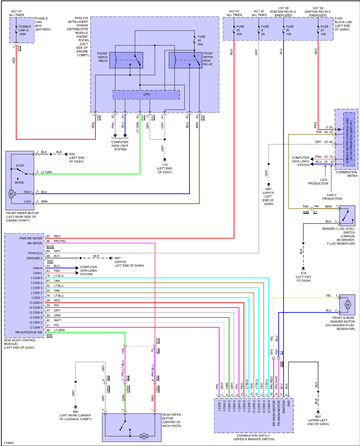
Fig 1: Wiper/Washer Circuit
