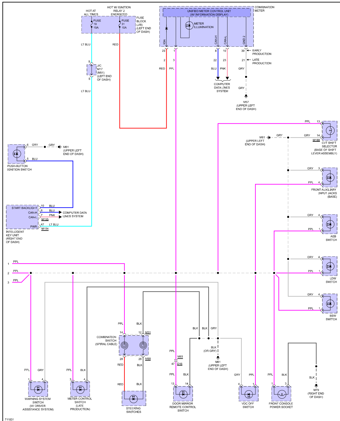
Fig 3: Instrument Illumination Circuit (2 of 2)
