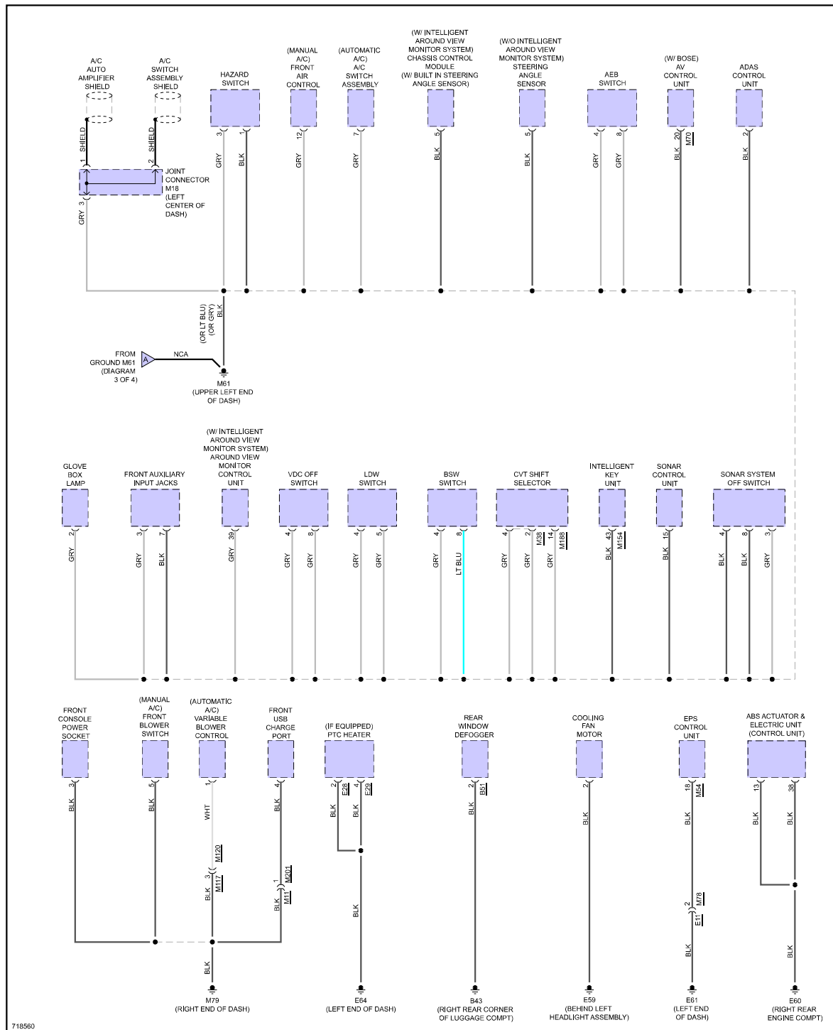
Fig 4: Ground Distribution Circuit (4 of 4)
