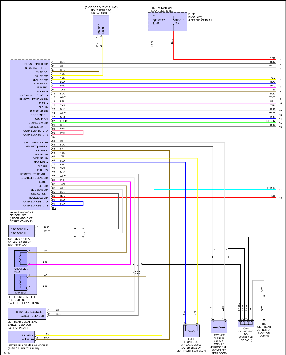
Fig 1: Supplemental Restraints Circuit (1 of 3)
