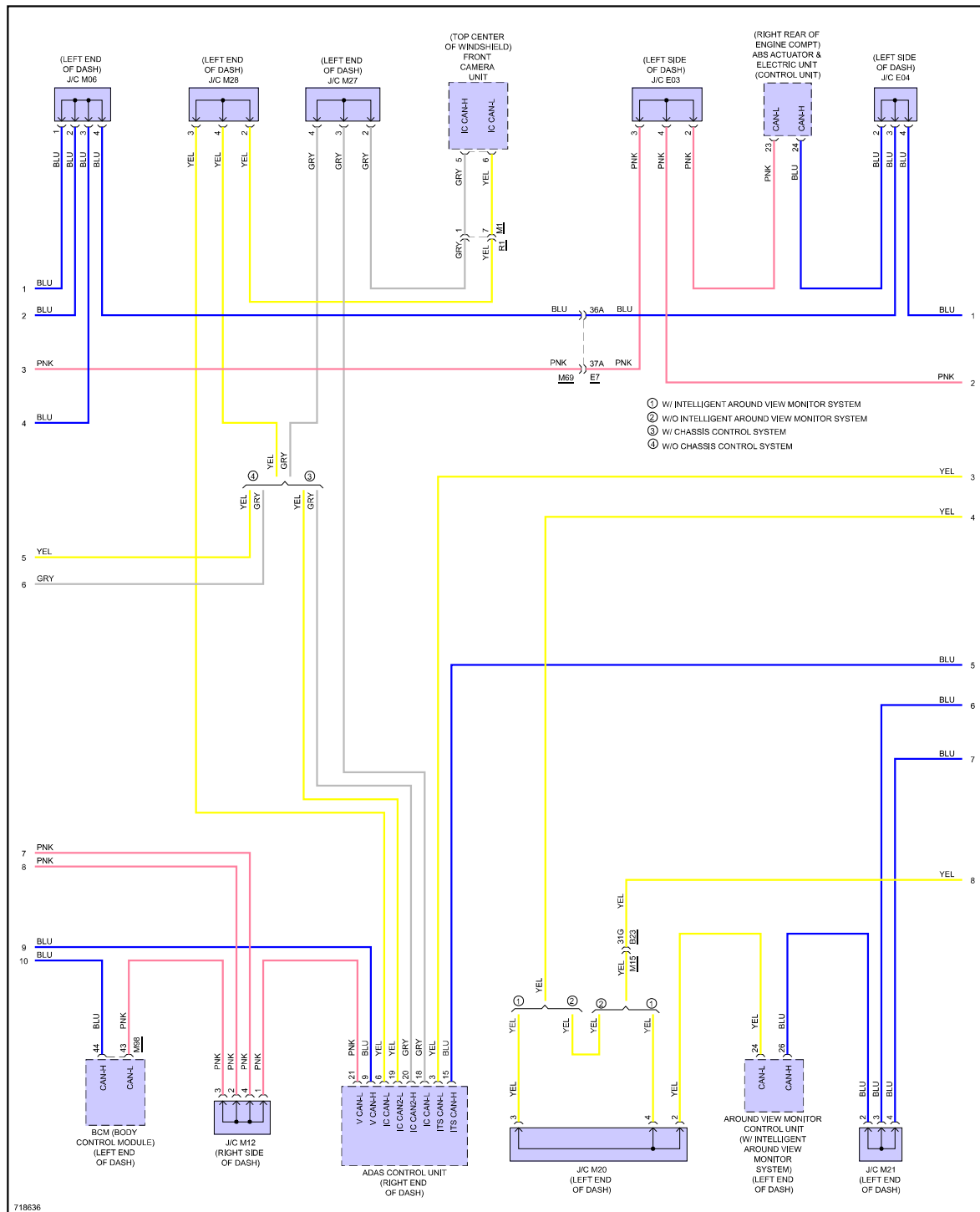
Fig 3: Computer Data Lines Circuit (3 of 4)
