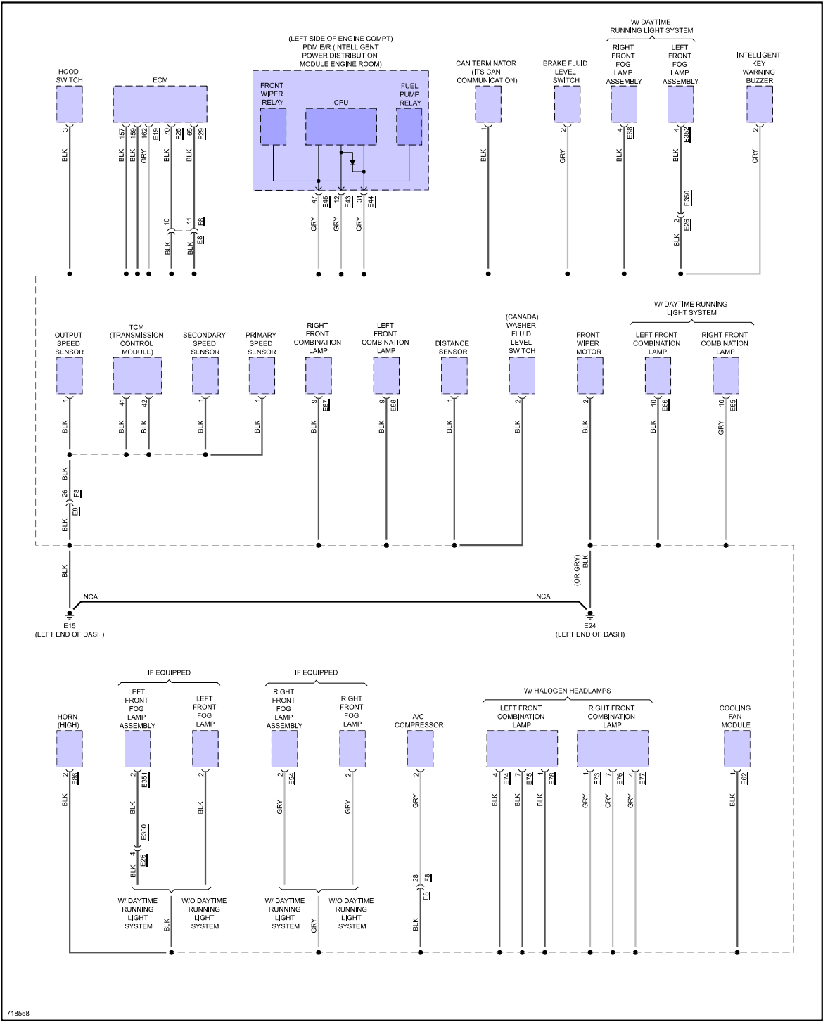
Fig 2: Ground Distribution Circuit (2 of 4)
