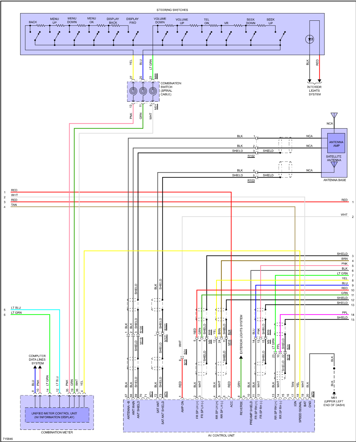
Fig 4: Premium Radio Circuit, W/ Bose (2 of 3)
