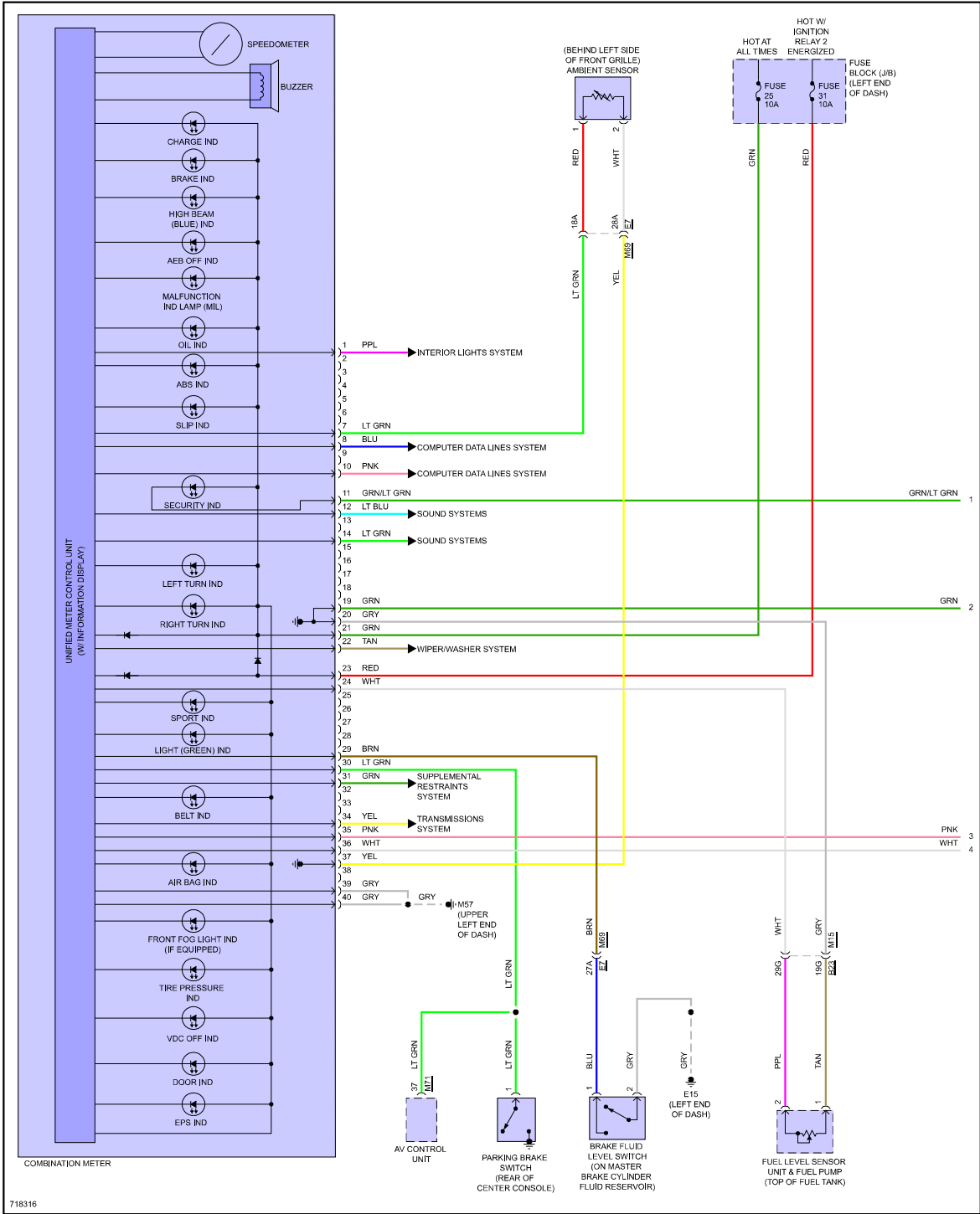
Fig 1: Instrument Cluster Circuit, Early Production (1 of 2)
