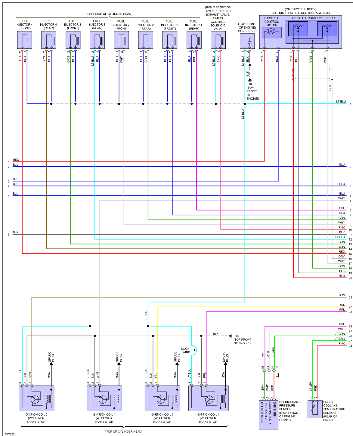
Fig 2: 1.6L, Engine Performance Circuit (2 of 6)
