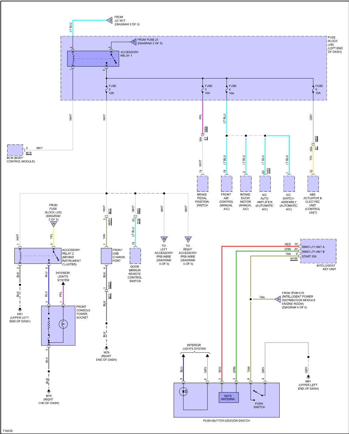
Fig 3: Power Distribution Circuit (3 of 5)
