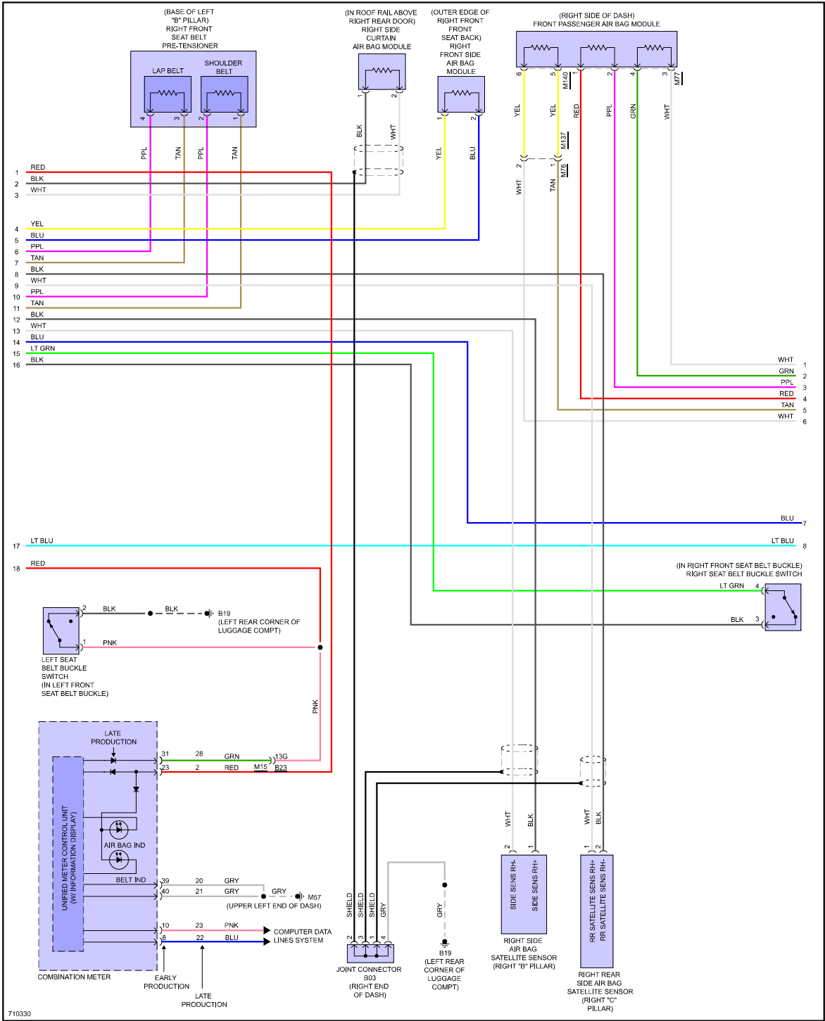
Fig 2: Supplemental Restraints Circuit (2 of 3)
