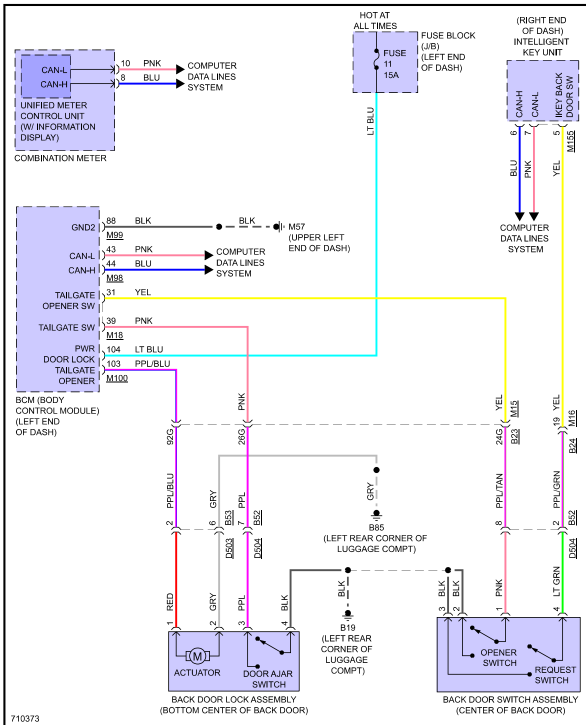
Fig 1: Back Door Opener Circuit
