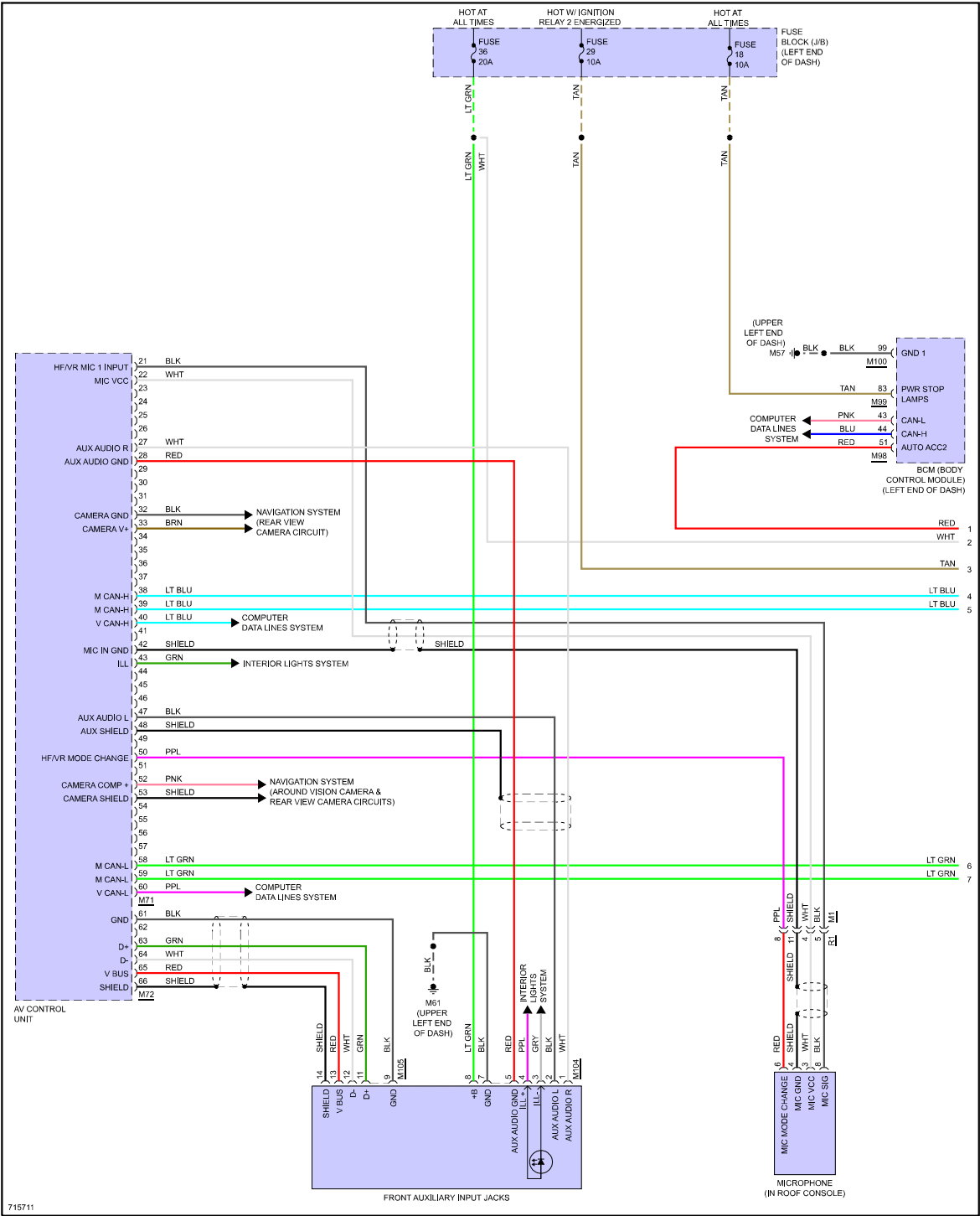
Fig 6: Navigation Circuit, W/O Bose (1 of 3)
